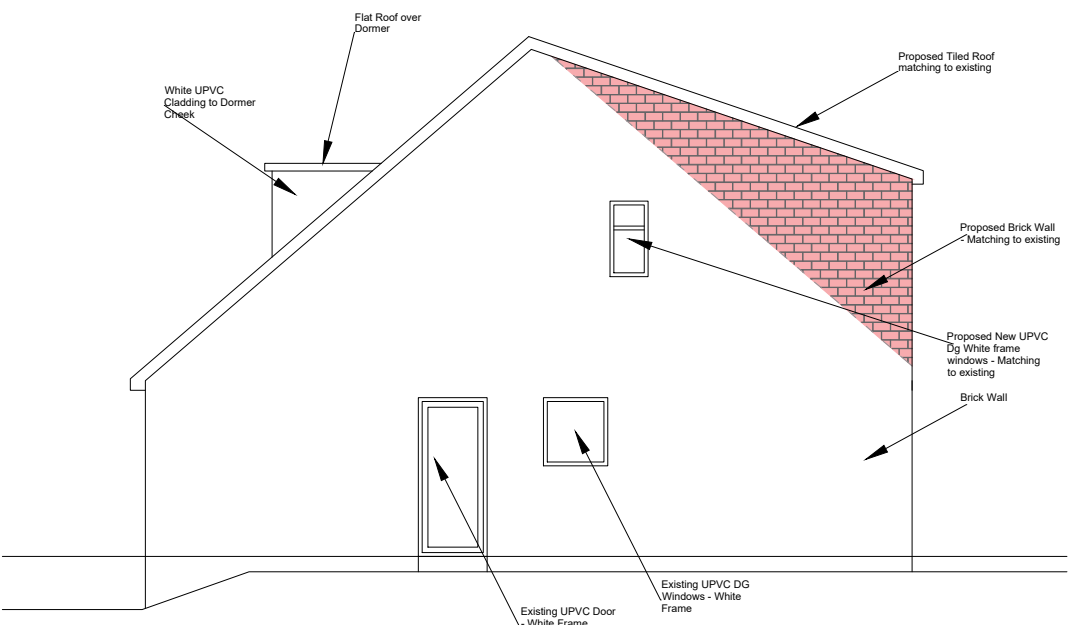
PROPOSED SIDE ELEVATION (South West)
