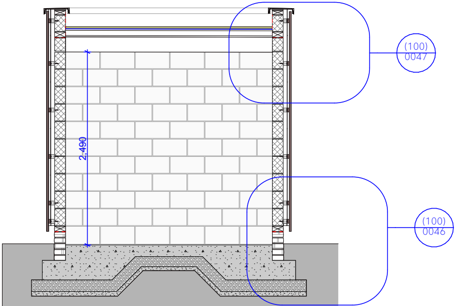
Section S-01
