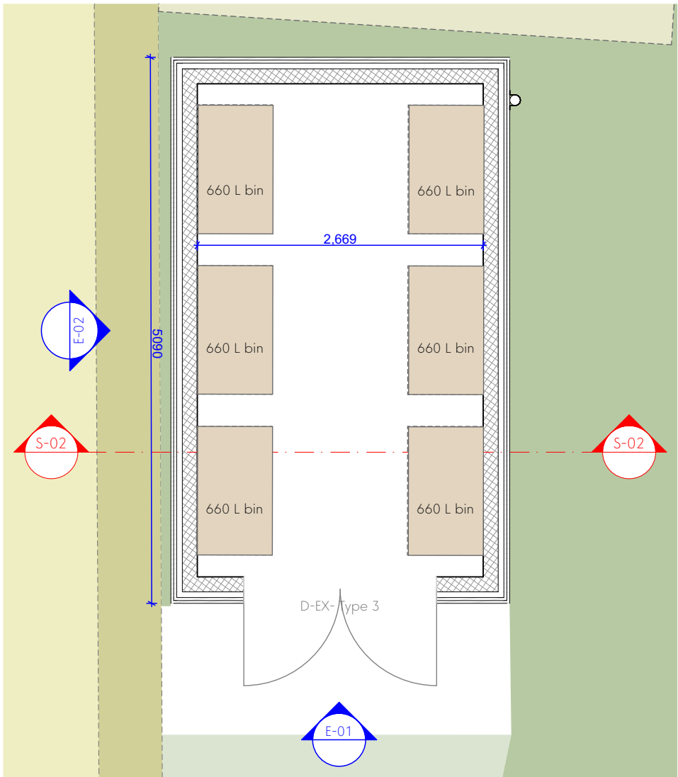
Floor Plan
