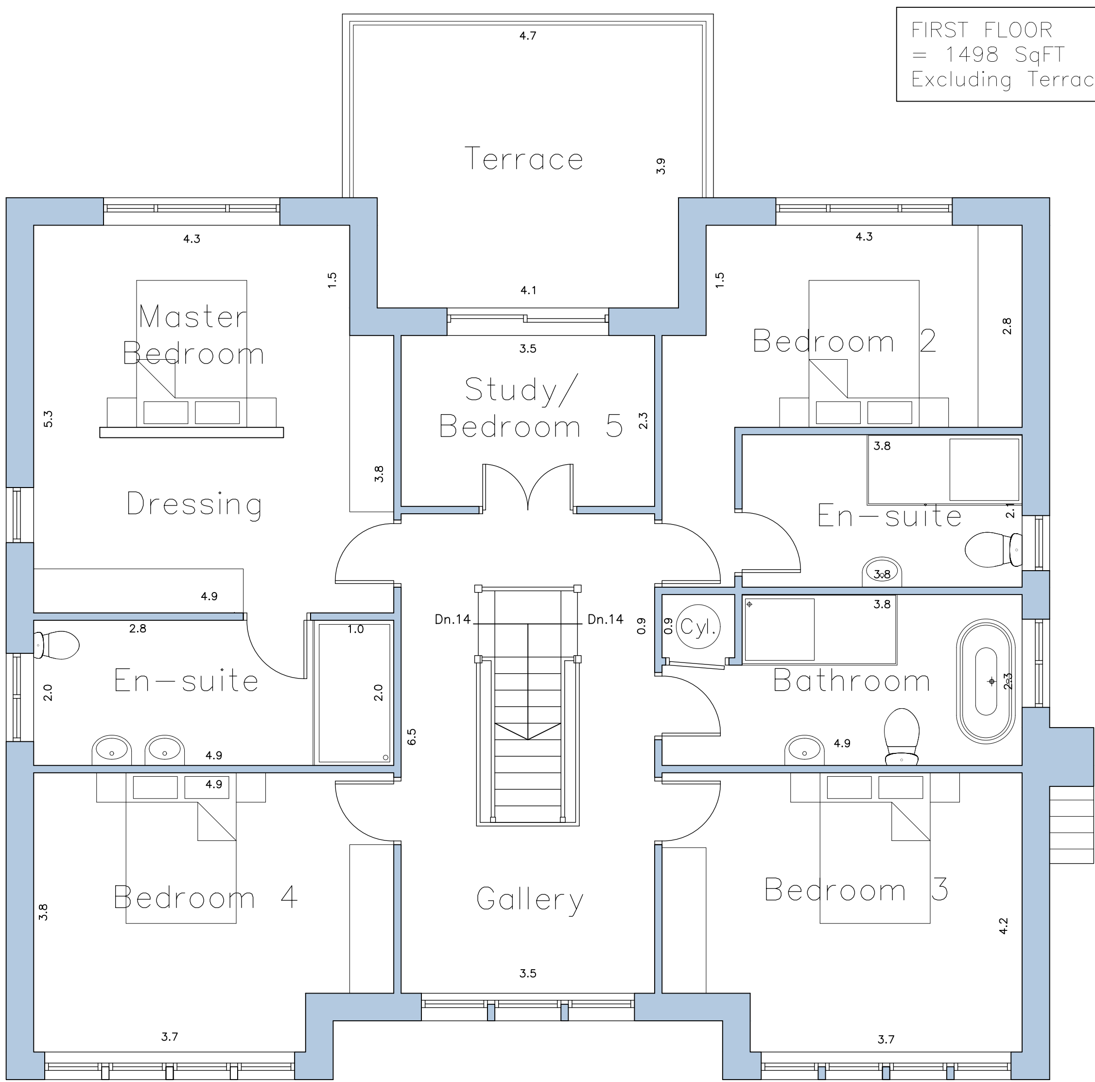
Proposed First Floor Layout Scale 1:50
