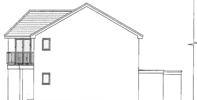
SIDE ELEVATION (WEST FACADE)
