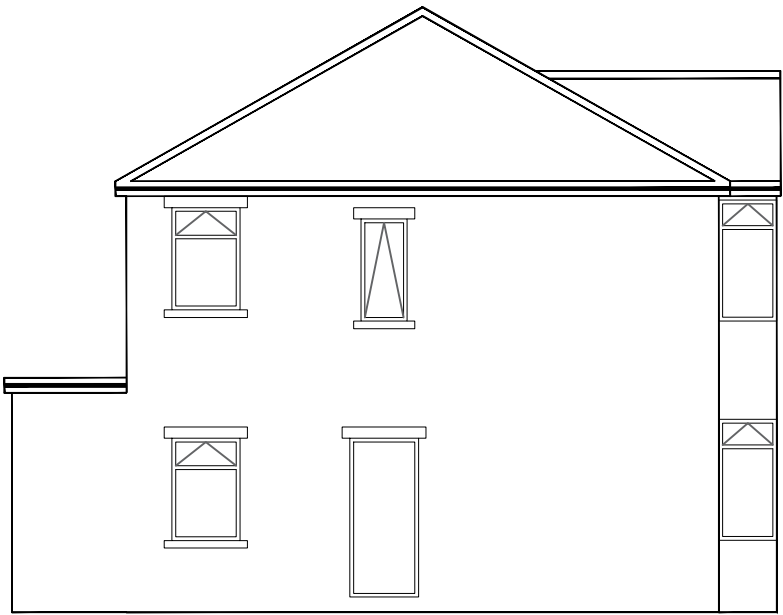
EXISTING SIDE ELEVATION (South)
