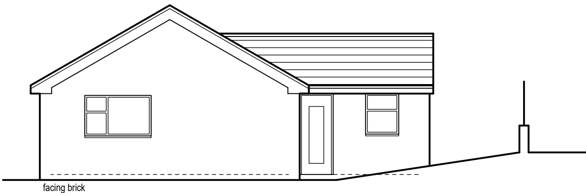
Proposed rear/north facing elevation (1:100)
