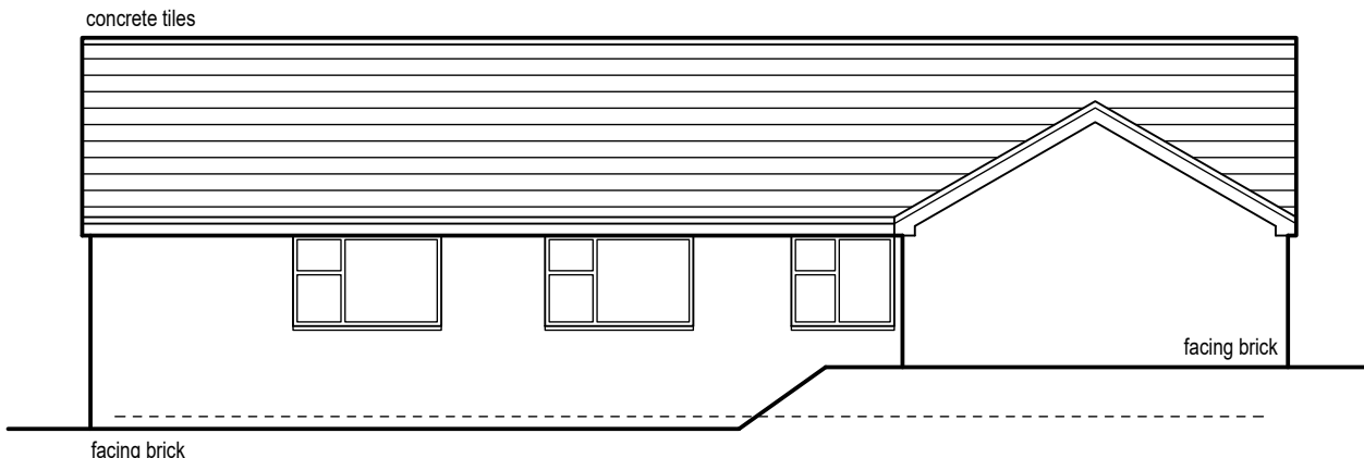
Proposed side/west facing elevation (1:100)
