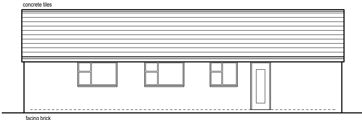
Existing side/west facing elevation (1:100)
