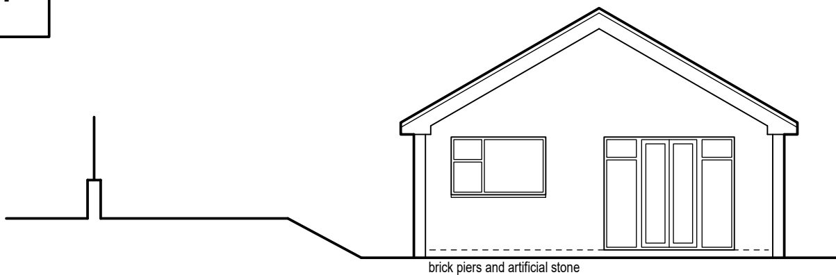
Existing front/south facing elevation (1:100)
