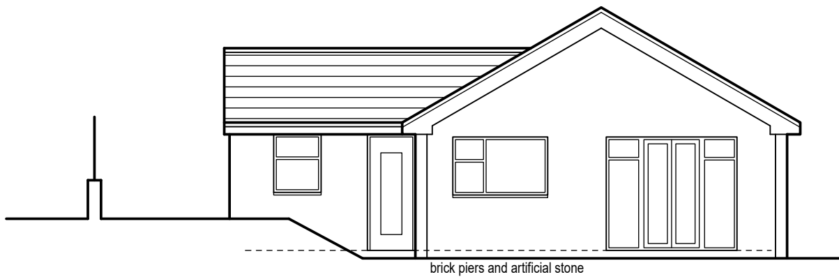
Proposed front/south facing elevation (1:100)
