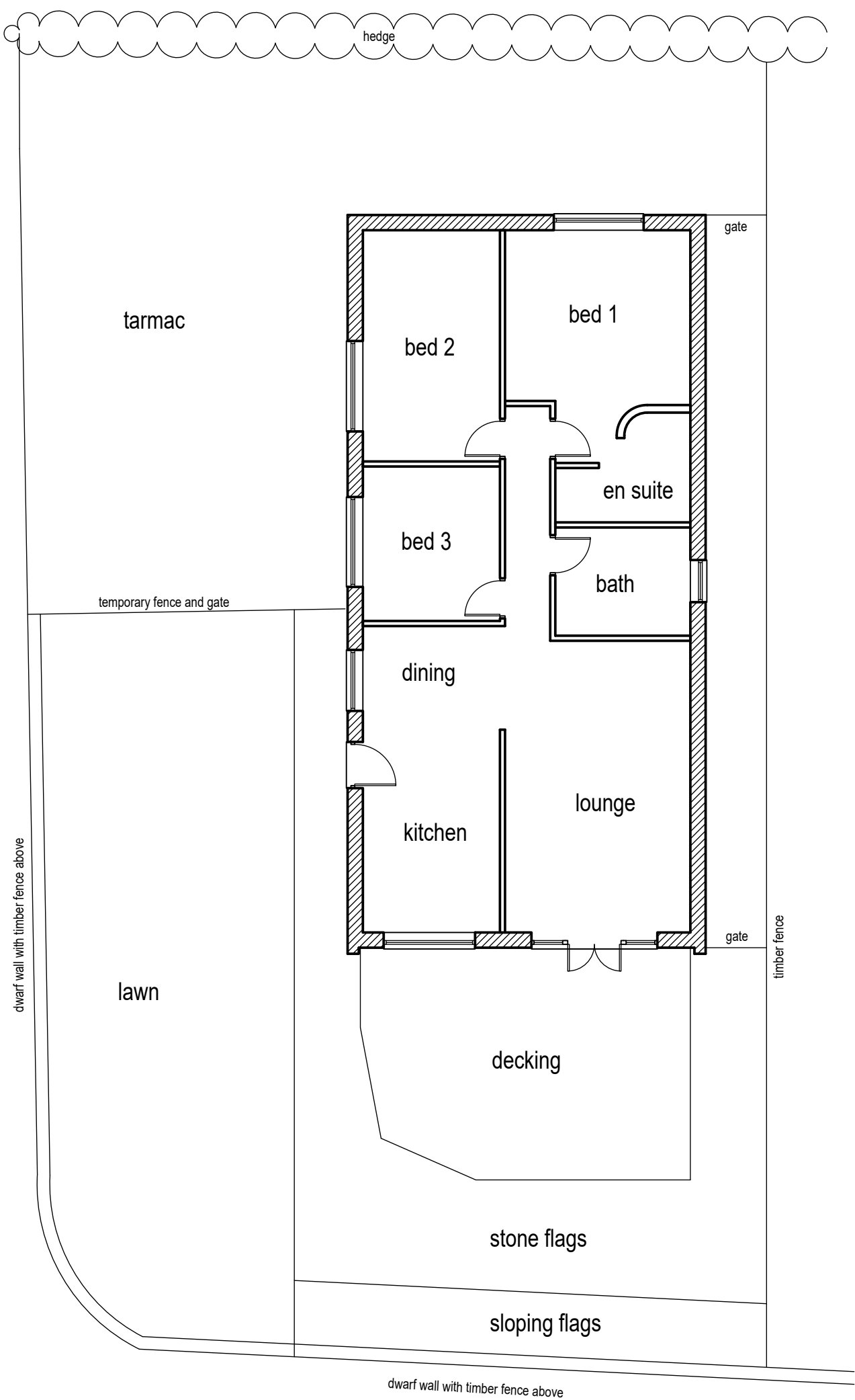
Existing floor layout (1:100)
