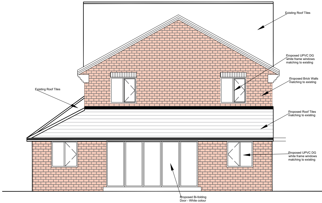
PROPOSED REAR ELEVATION (South)
