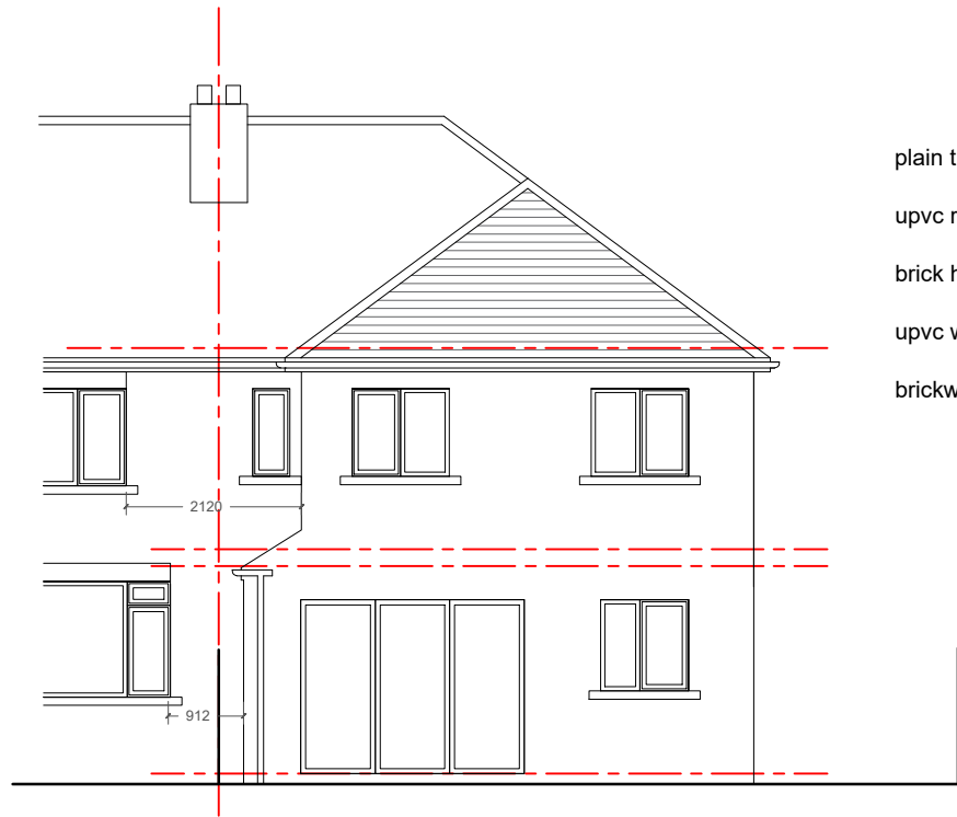
North Elevation
