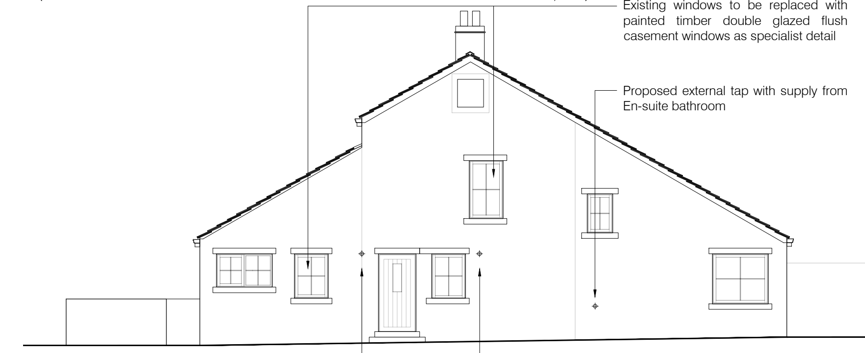
North-Western Elevation 1: 100
