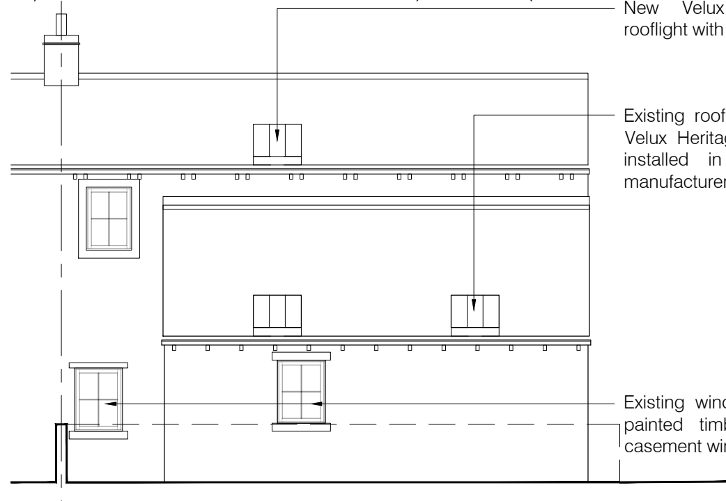
North-Eastern Elevation 1: 100
