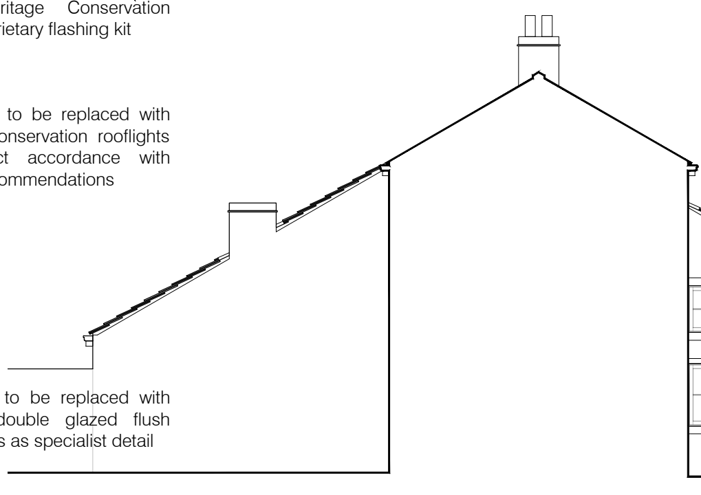
South-Eastern Elevation 1: 100
