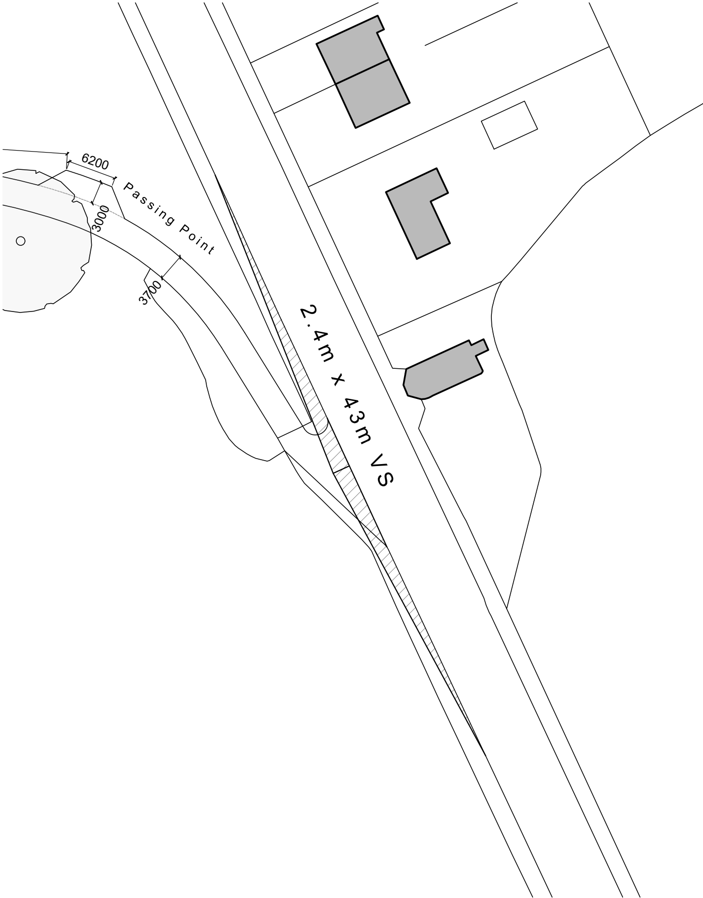
VISIBILITY SPLAY 1:500 @ A1
