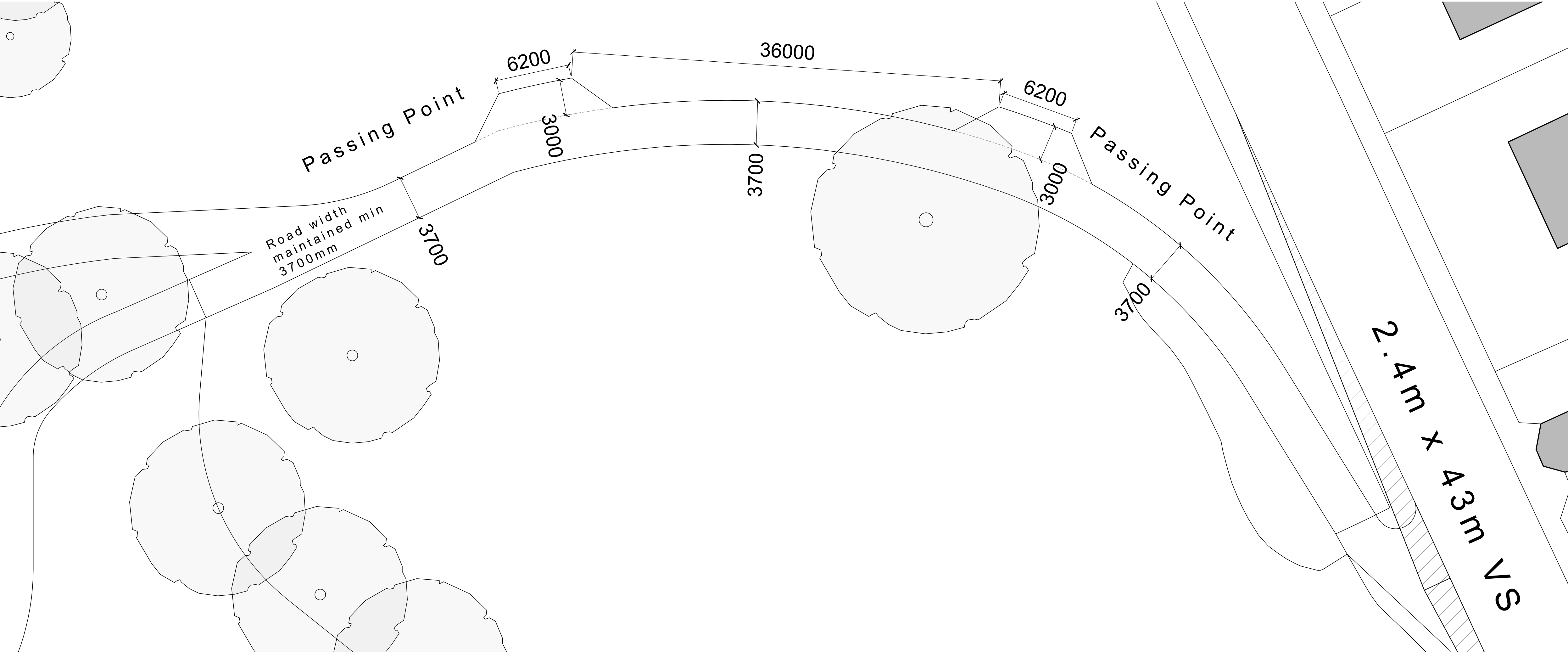
PASSING ZONES AND ROAD WIDTH 1:100 @ A1
