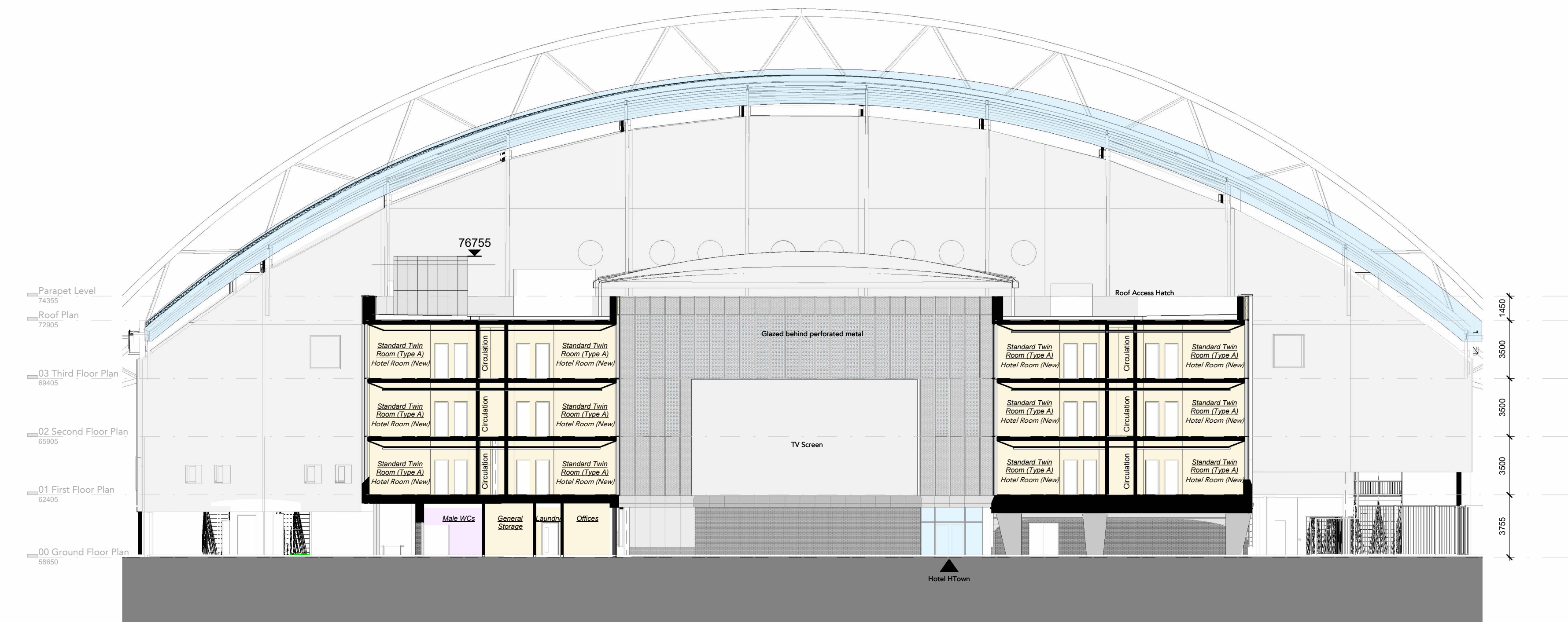
BB Proposed Section BB 1:200
