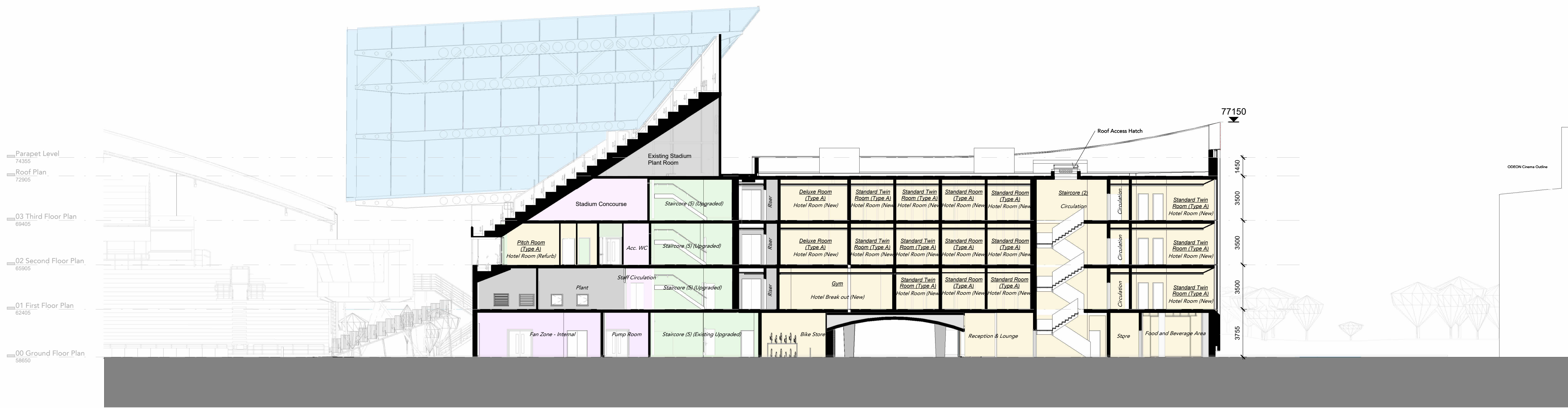
AA Proposed Section AA 1:200
