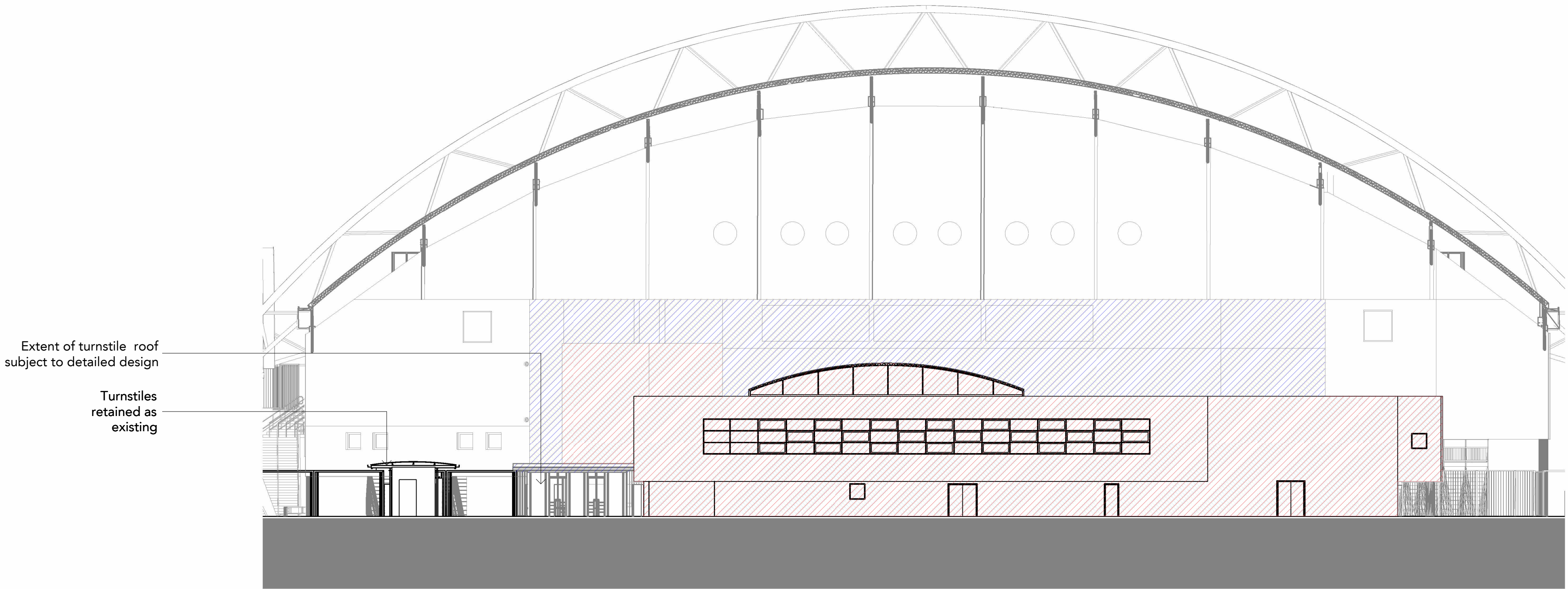
2 Existing North Eastern Elevation - Demo 1 : 200
