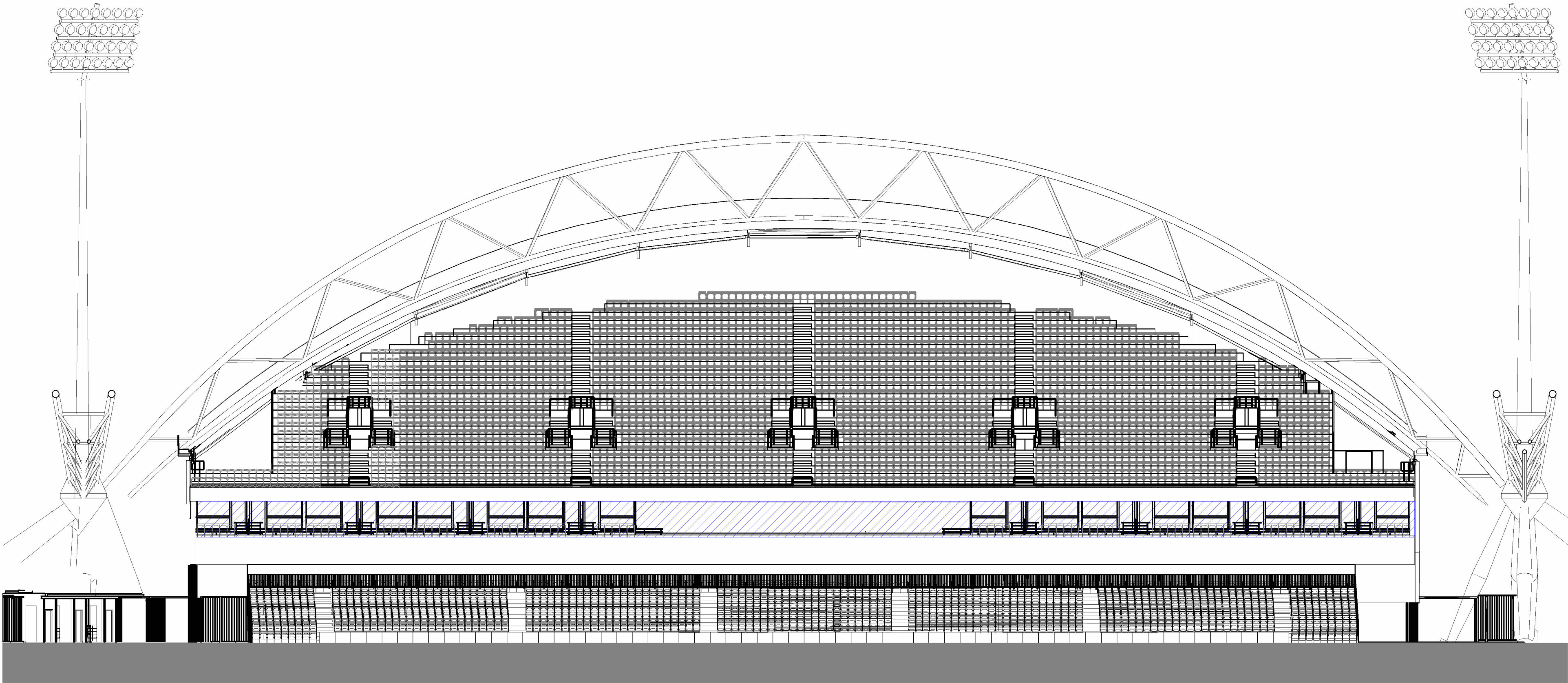
3 Existing South Western Elevation - Demo 1 : 200
