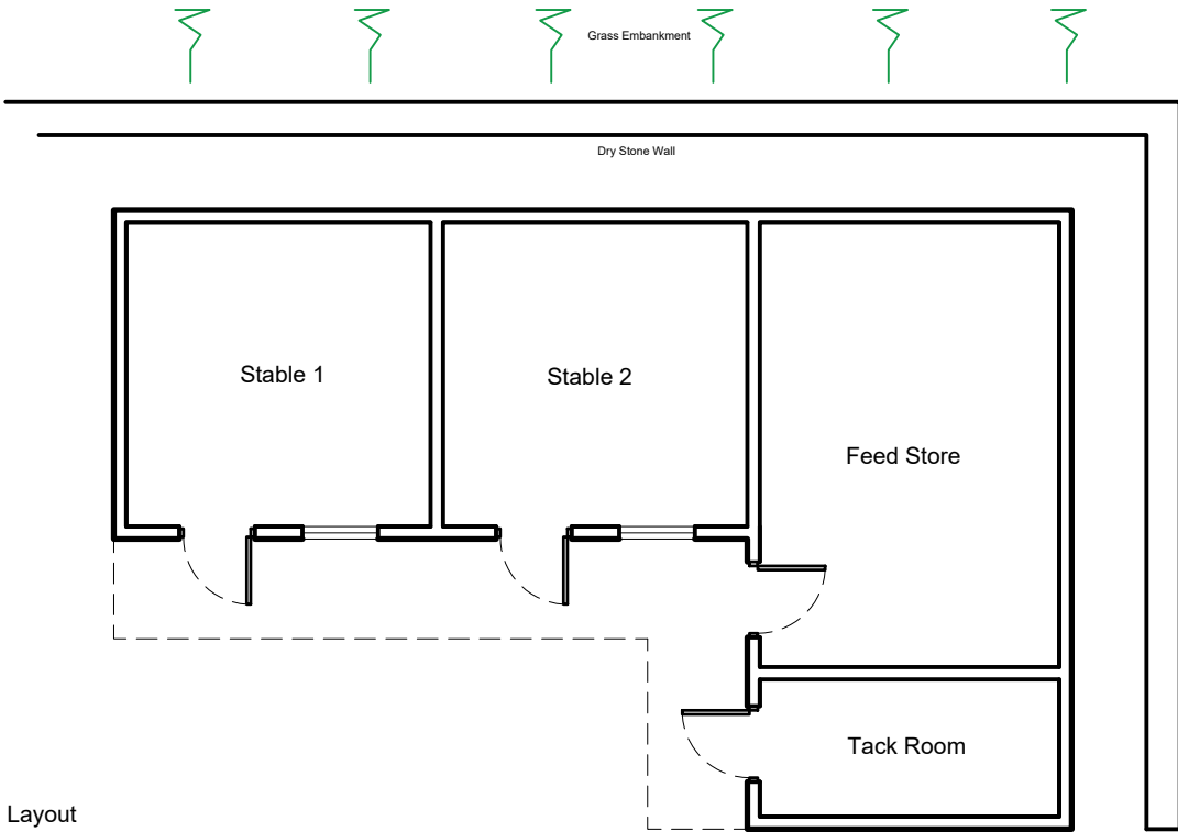
Stable Layout
