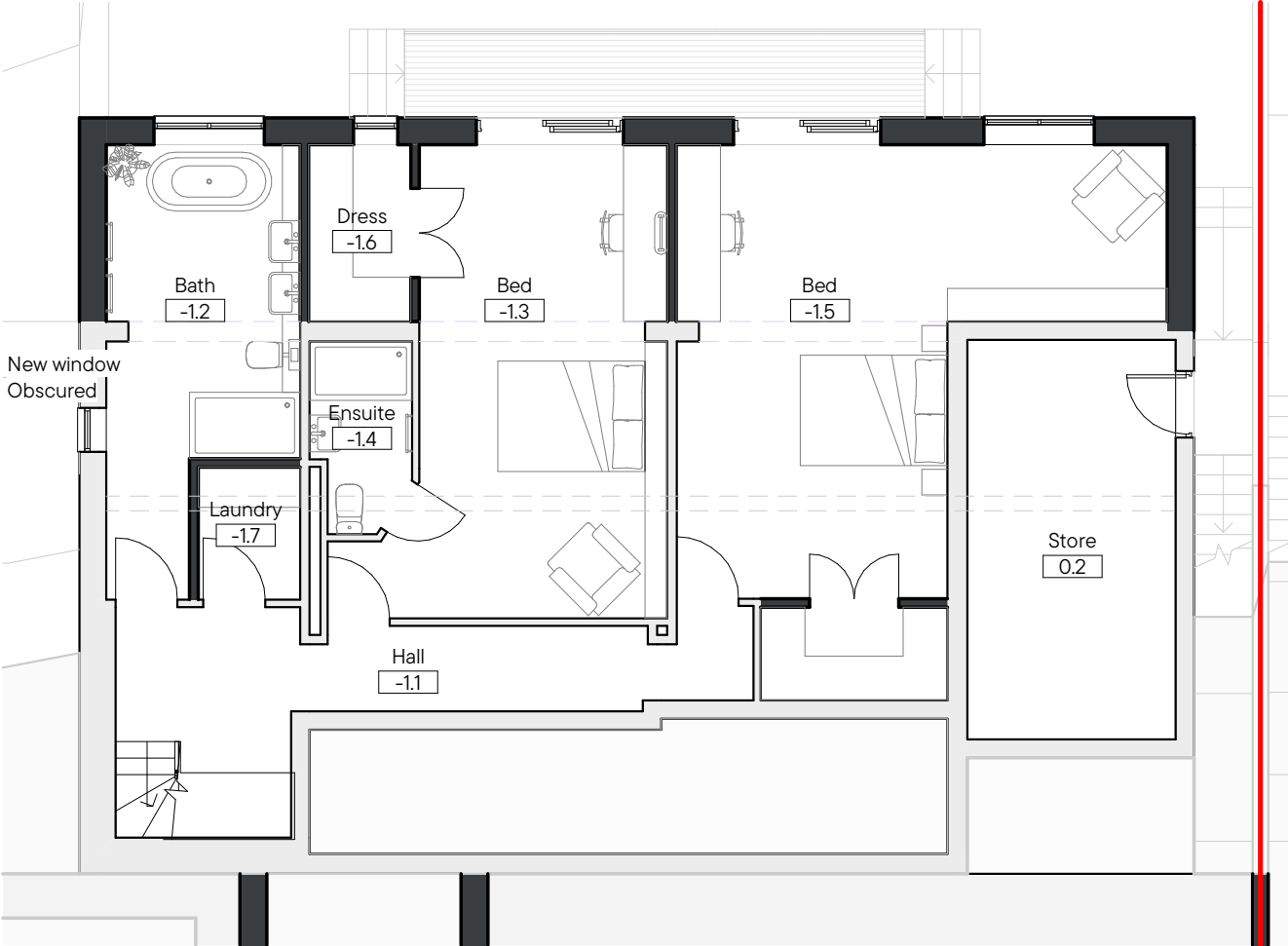
-1 Lower Ground 1:100
