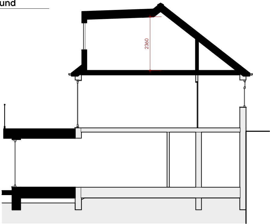
A Section A 1:100
