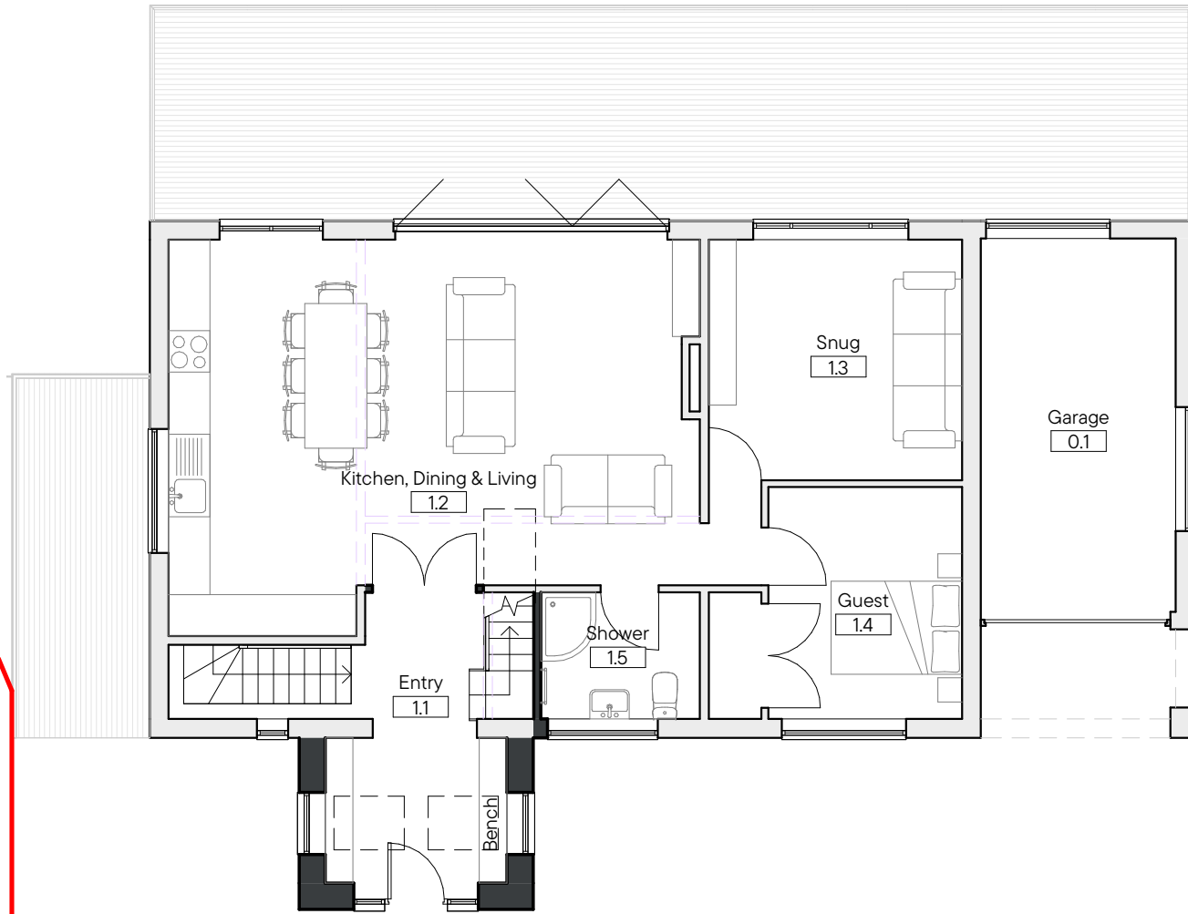
1 Ground 1:100
