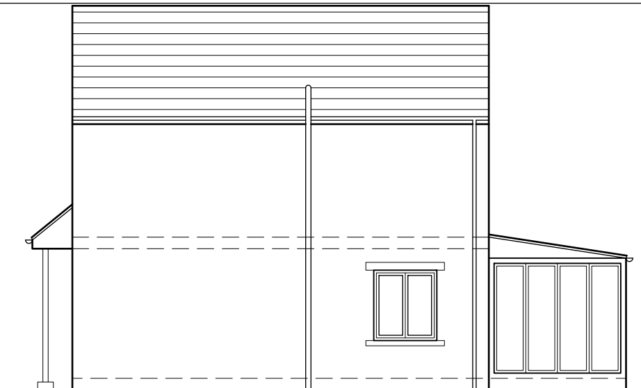
East Elevation
