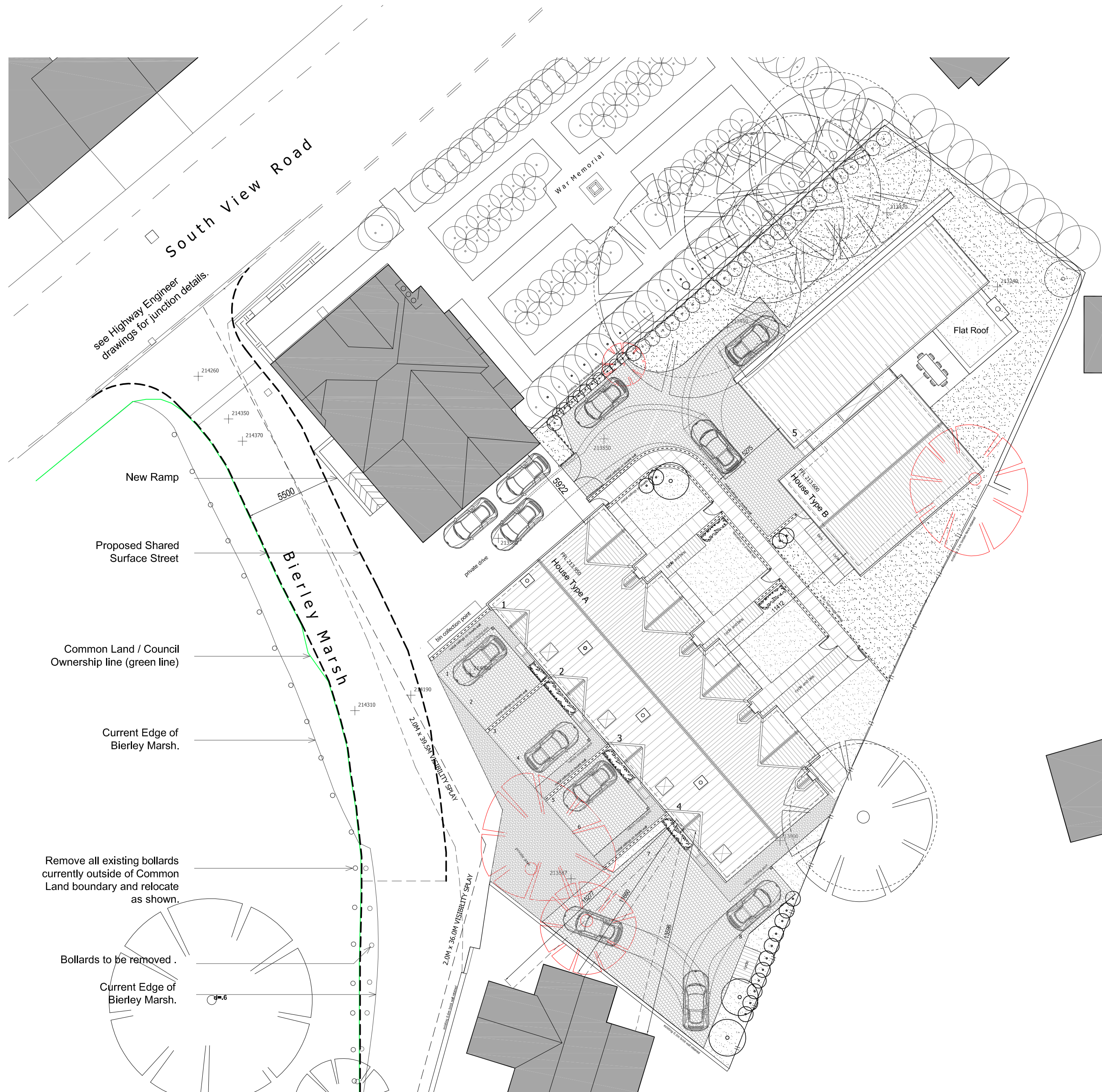
proposed site layout. scale 1 : 200 @ A2
