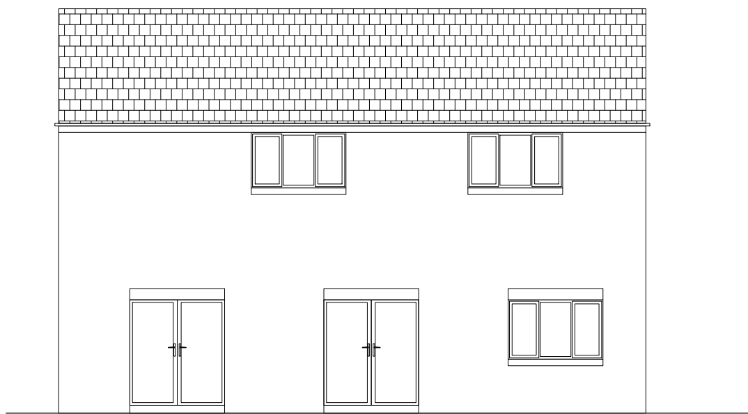
EXISTING FRONT ELEVATION Scale 1:100@A1
