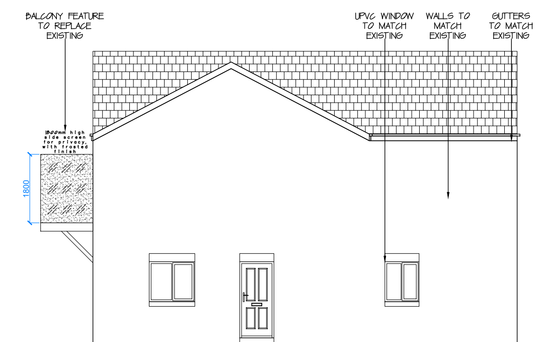
PROPOSED REAR ELEVATION Scale 1:100@A1
