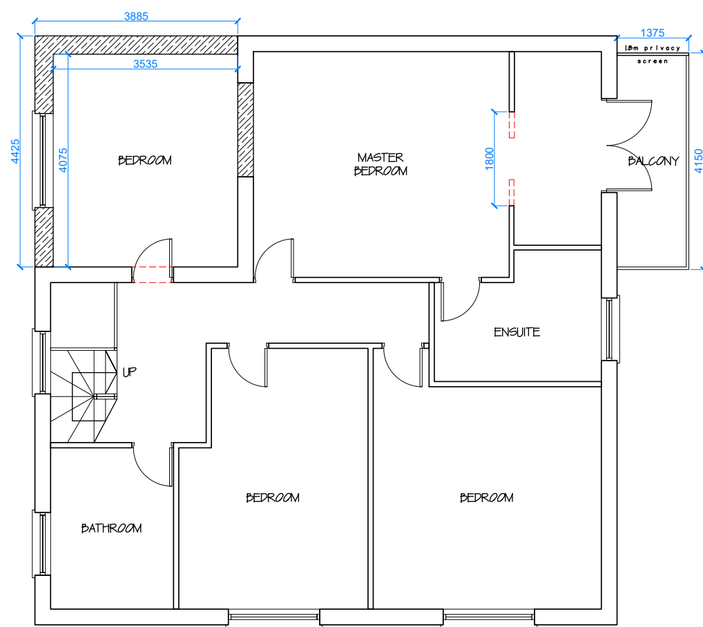
PROPOSED FIRST FLOOR Scale 1:100@A1
