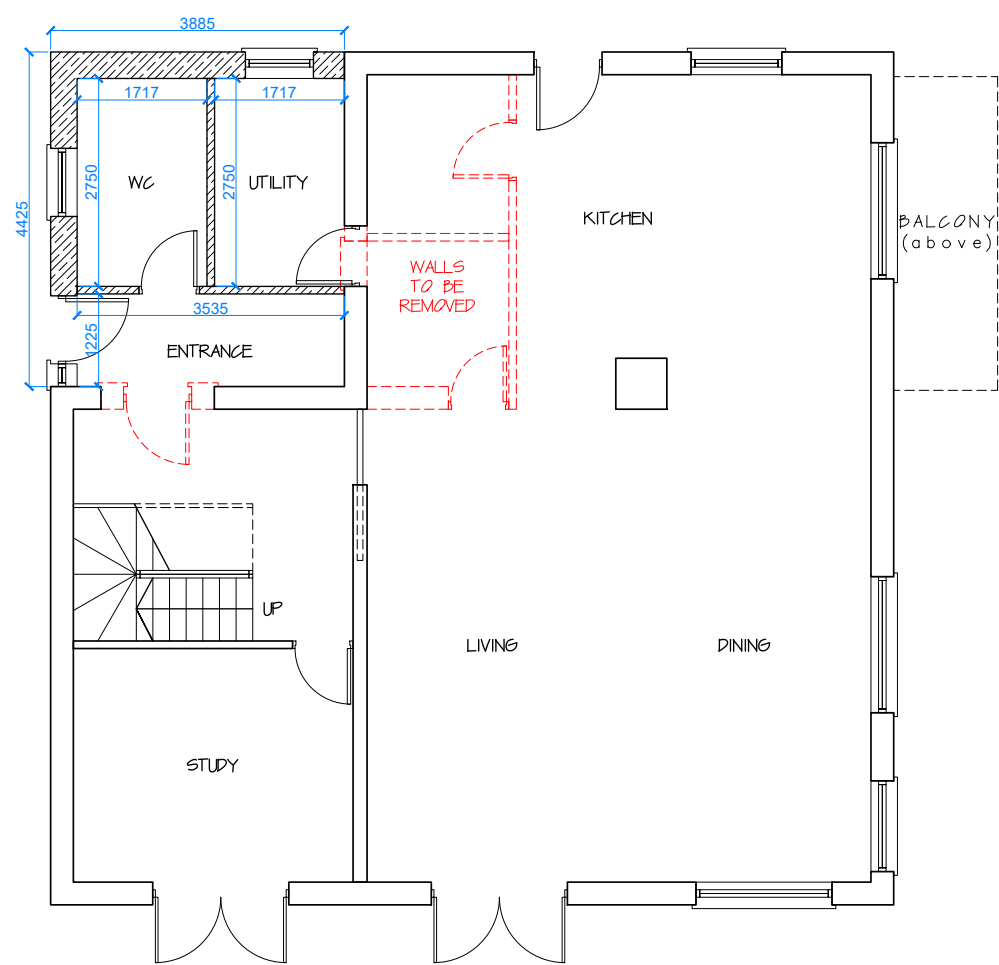
PROPOSED GROUND FLOOR Scale 1:100@A1
