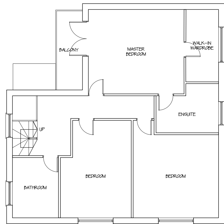
EXISTING FIRST FLOOR Scale 1:100@A1
