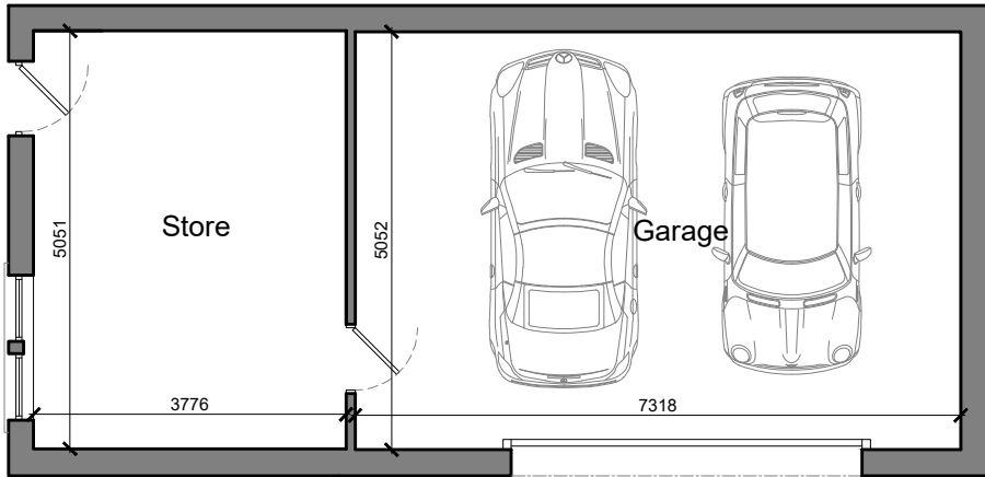
AS-APPROVED GARAGE FLOOR PLAN SCALE - 1:100
