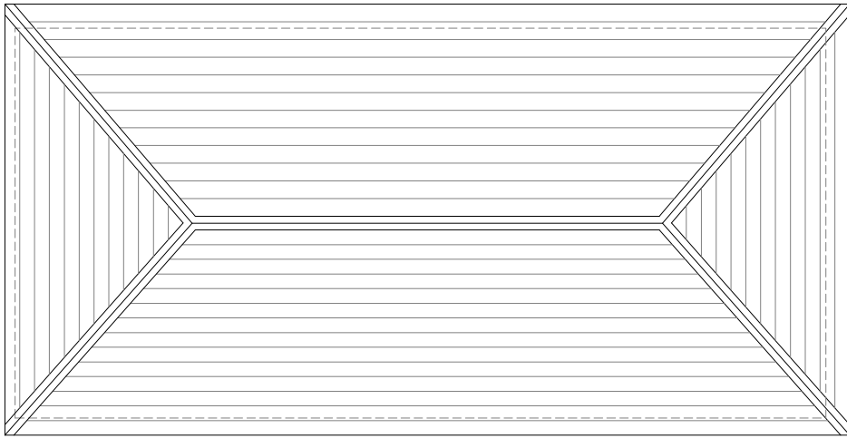
AS-APPROVED GARAGE ROOF PLAN SCALE - 1:100
