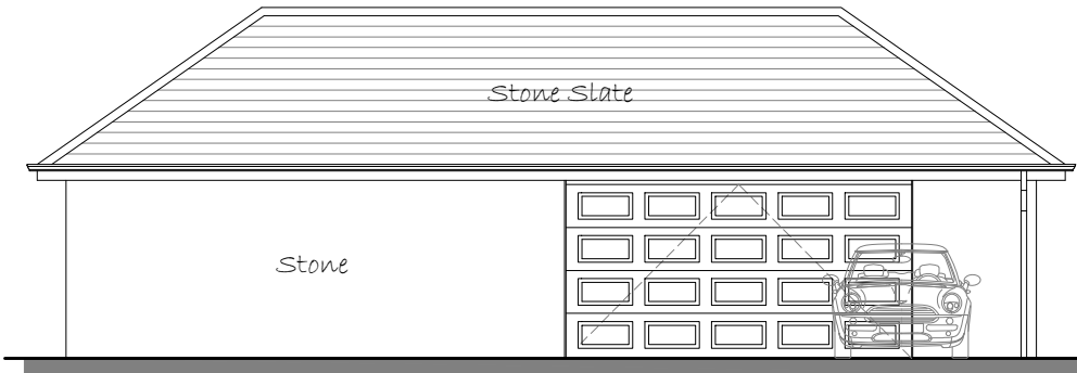
AS-APPROVED NORTH-EAST ELEVATION SCALE - 1:100
