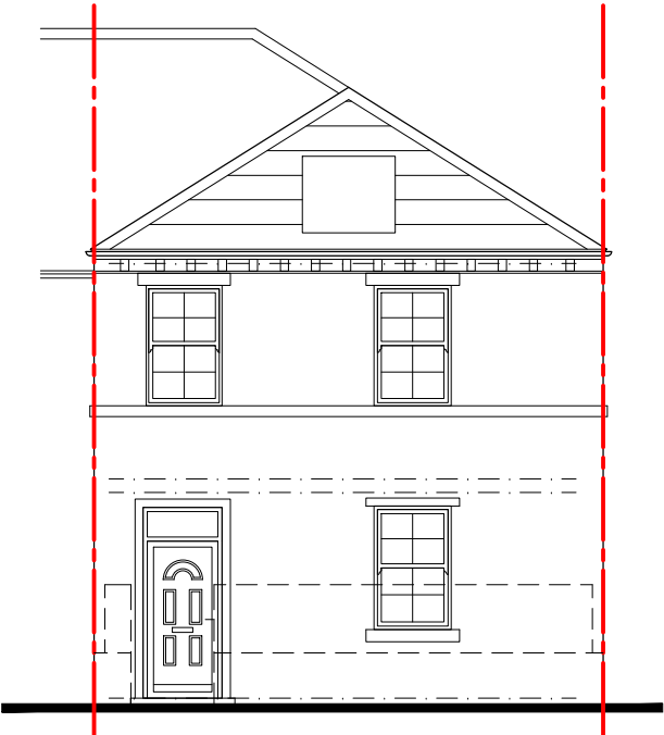
Front Elevation As Proposed
