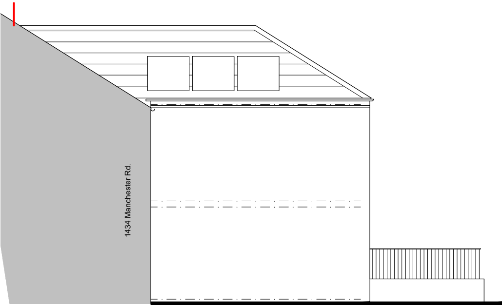
West Elevation As Proposed
