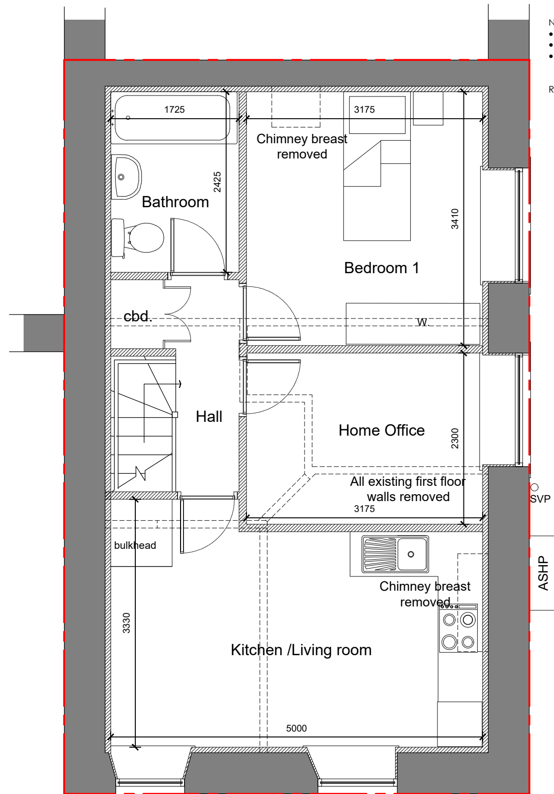
First Floor Flat 2 As Proposed (48.9m 2 )
