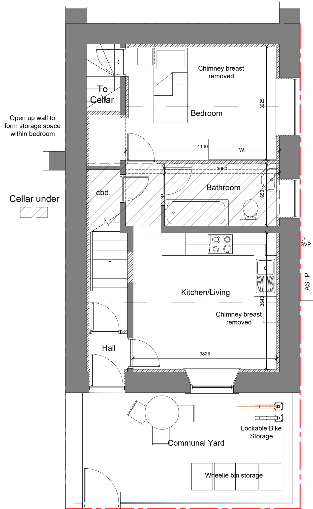
Ground Floor Flat 1 As Proposed (40m 2 )
