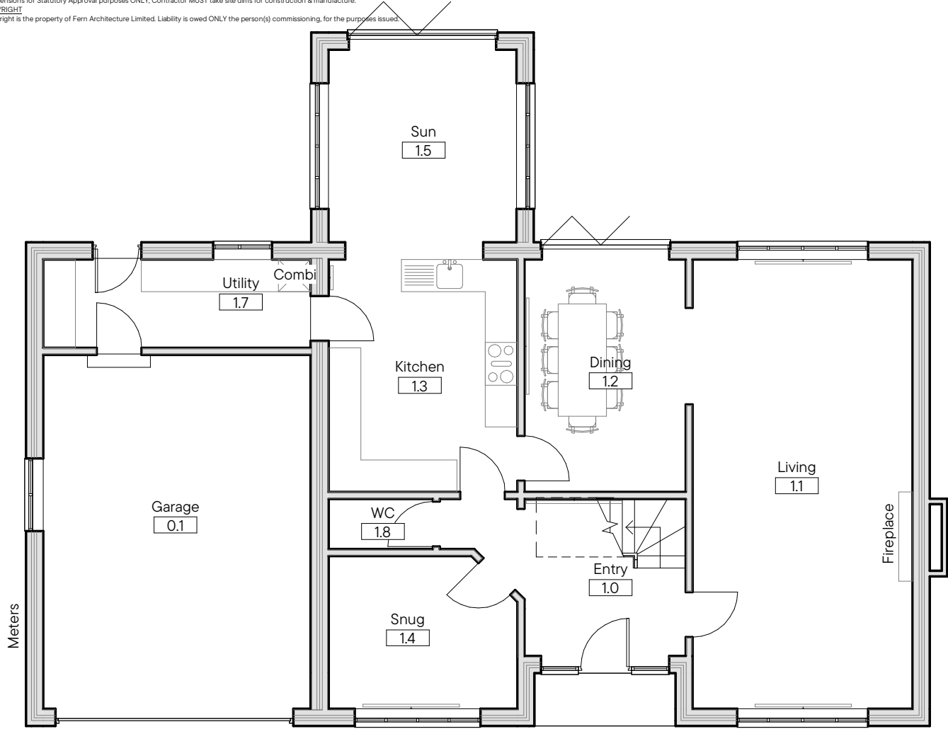
1 1 Ground 1:100
