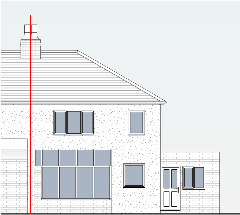
N Rear 1:100
