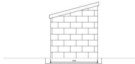
Side elevation 2 1 : 25
