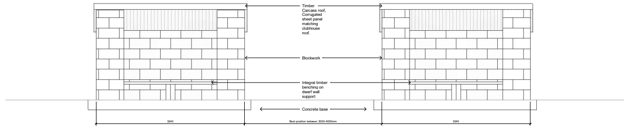
Front Elevation 1 : 25
