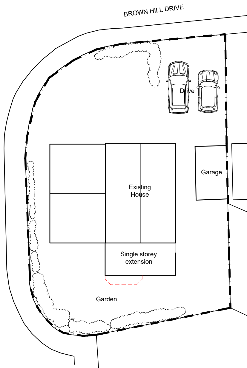
PROPOSED SITE LAYOUT (1:200)
