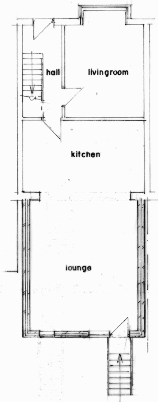
GROUND FLOOR PLAN (PROPOSED)
