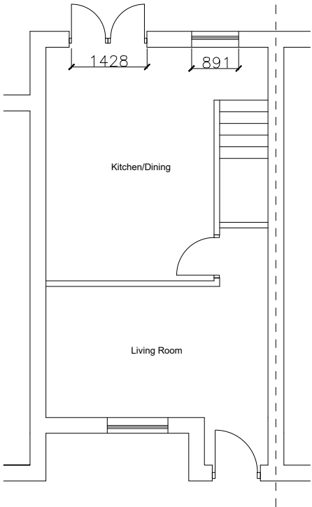
EXISTING GROUND FLOOR PLAN
