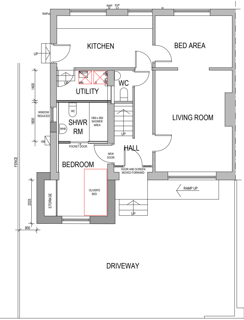
PART BLOCK PLAN 1:100
