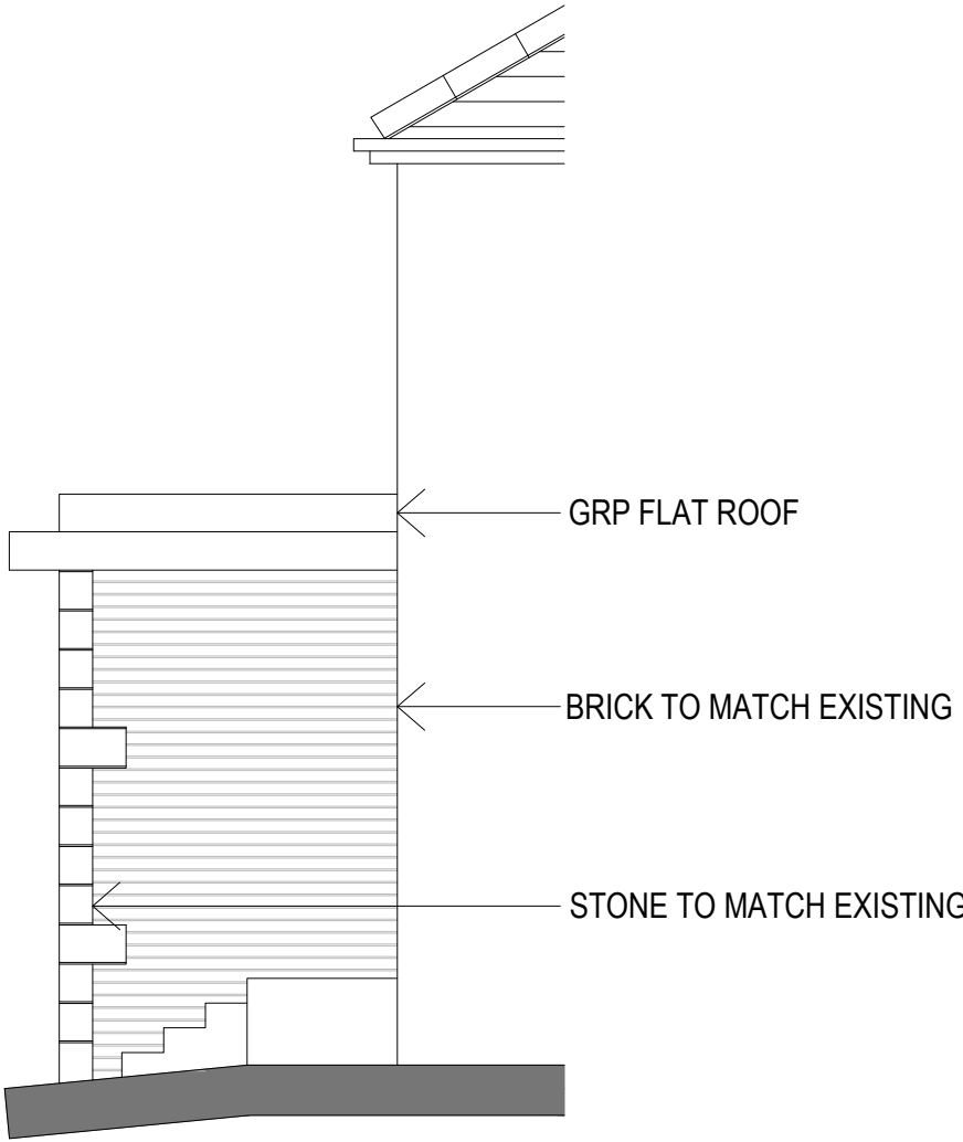
1:50 NORTH WEST ELEVATION
