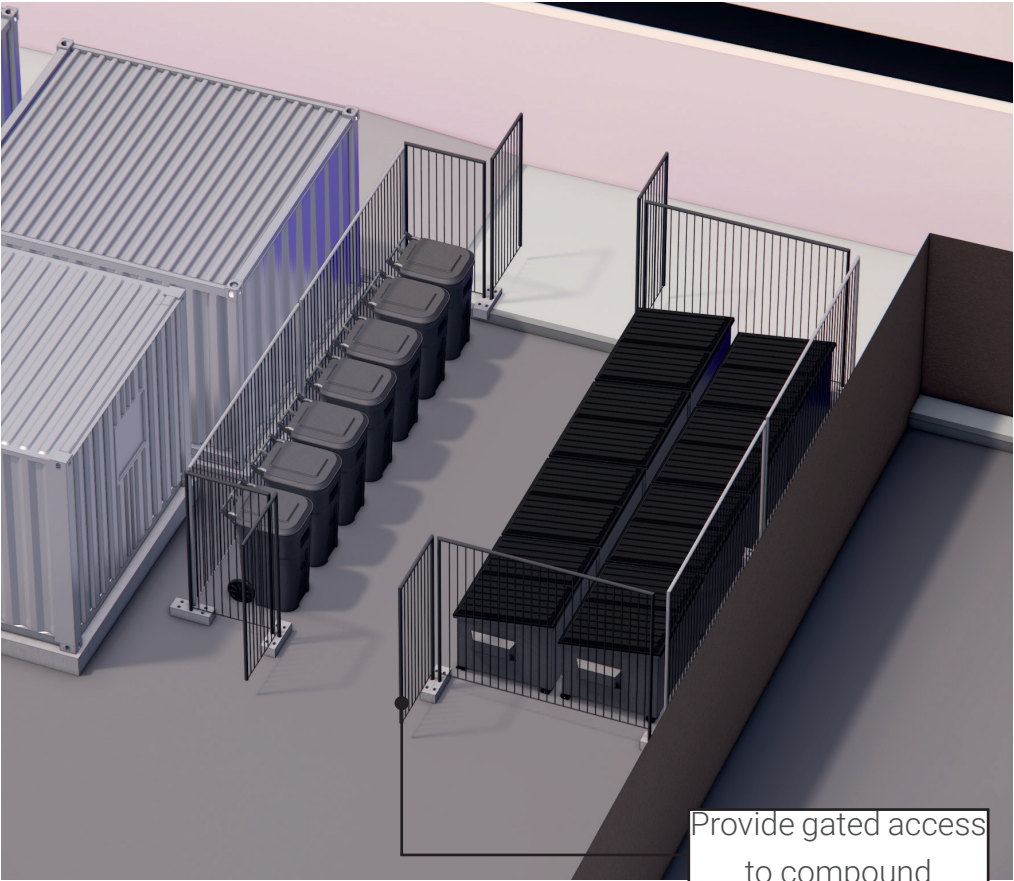
Waste Storage 3D View
