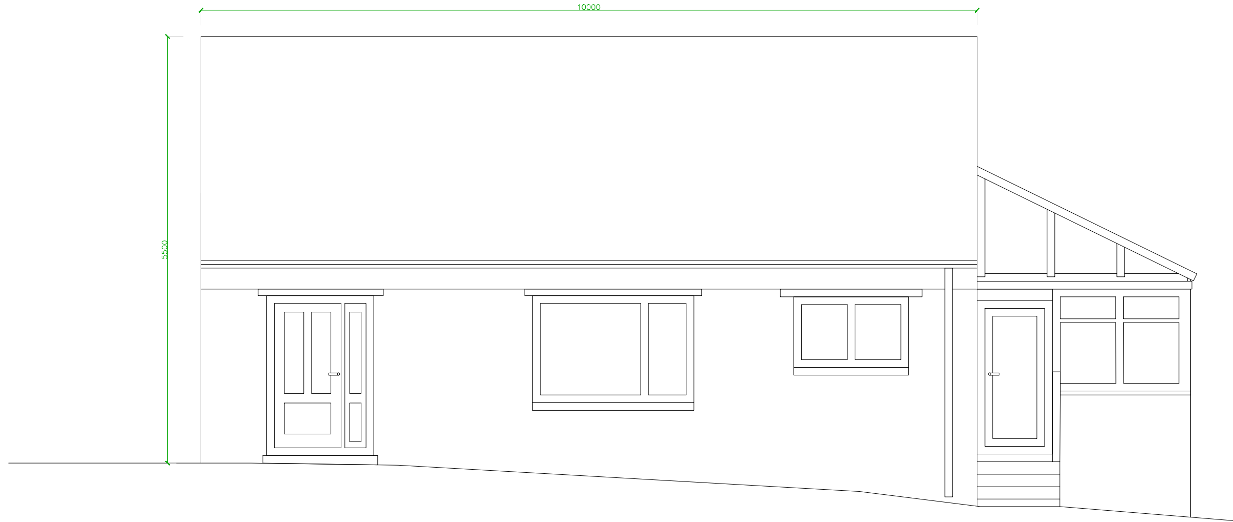
EXISTING FRONT - SOUTH ELEVATION (BANK END ROAD ELEVATION) SCALE: 1:50 @ A3
