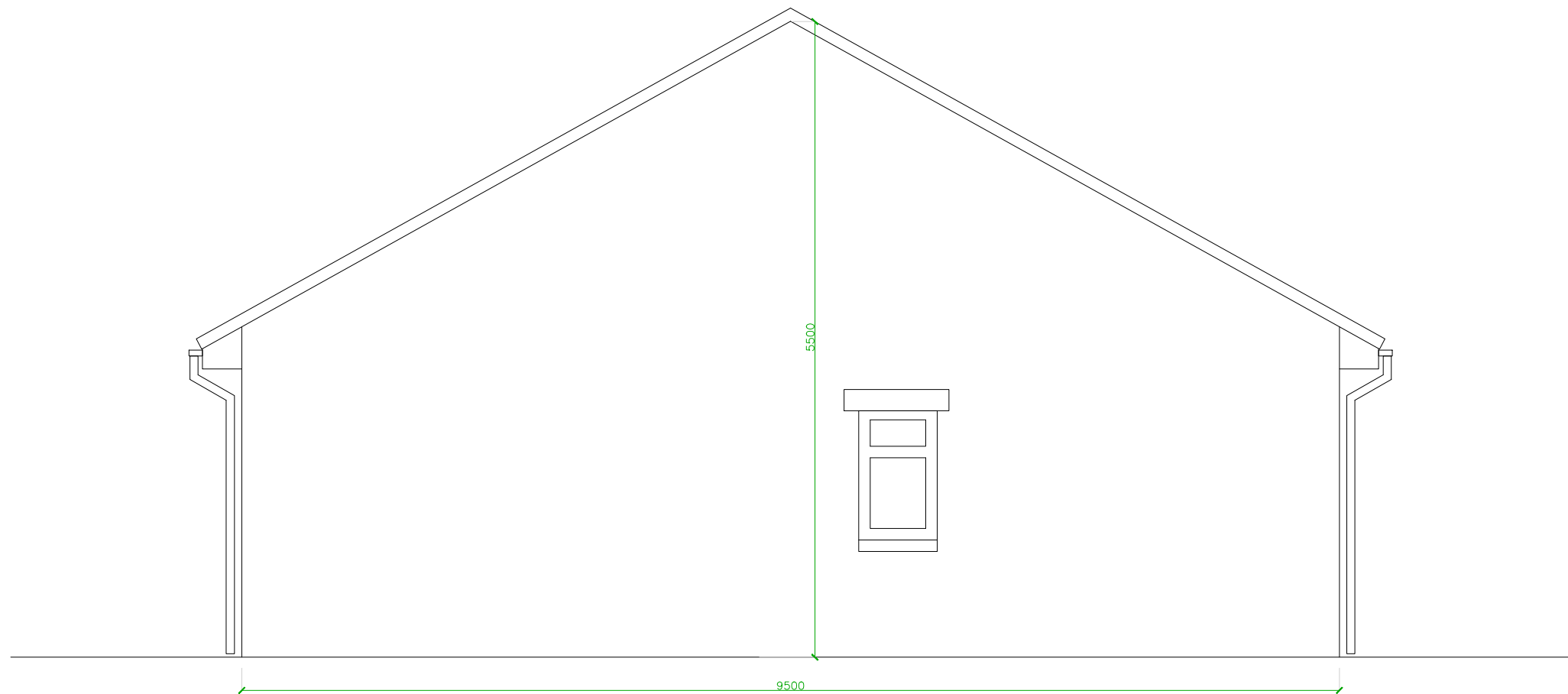
PROPOSED WEST ELEVATION SCALE: 1:50 @ A3
