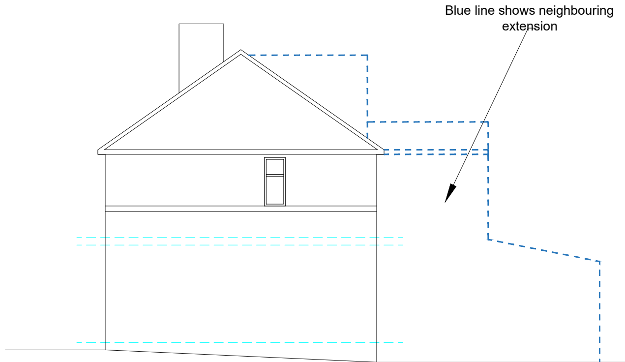
EXISTING SIDE ELEVATION (North West)
