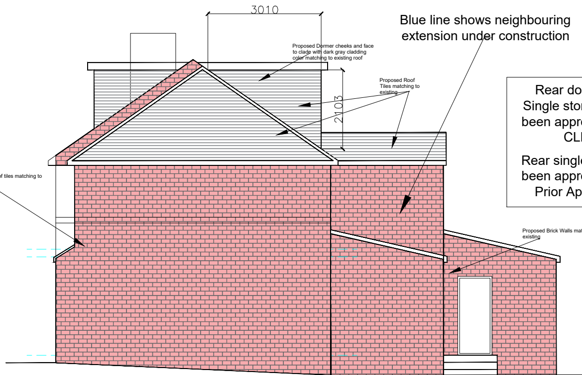
PROPOSED SIDE ELEVATION (North West)
