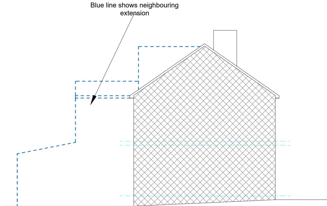
PROPOSED SIDE ELEVATION (South East)
