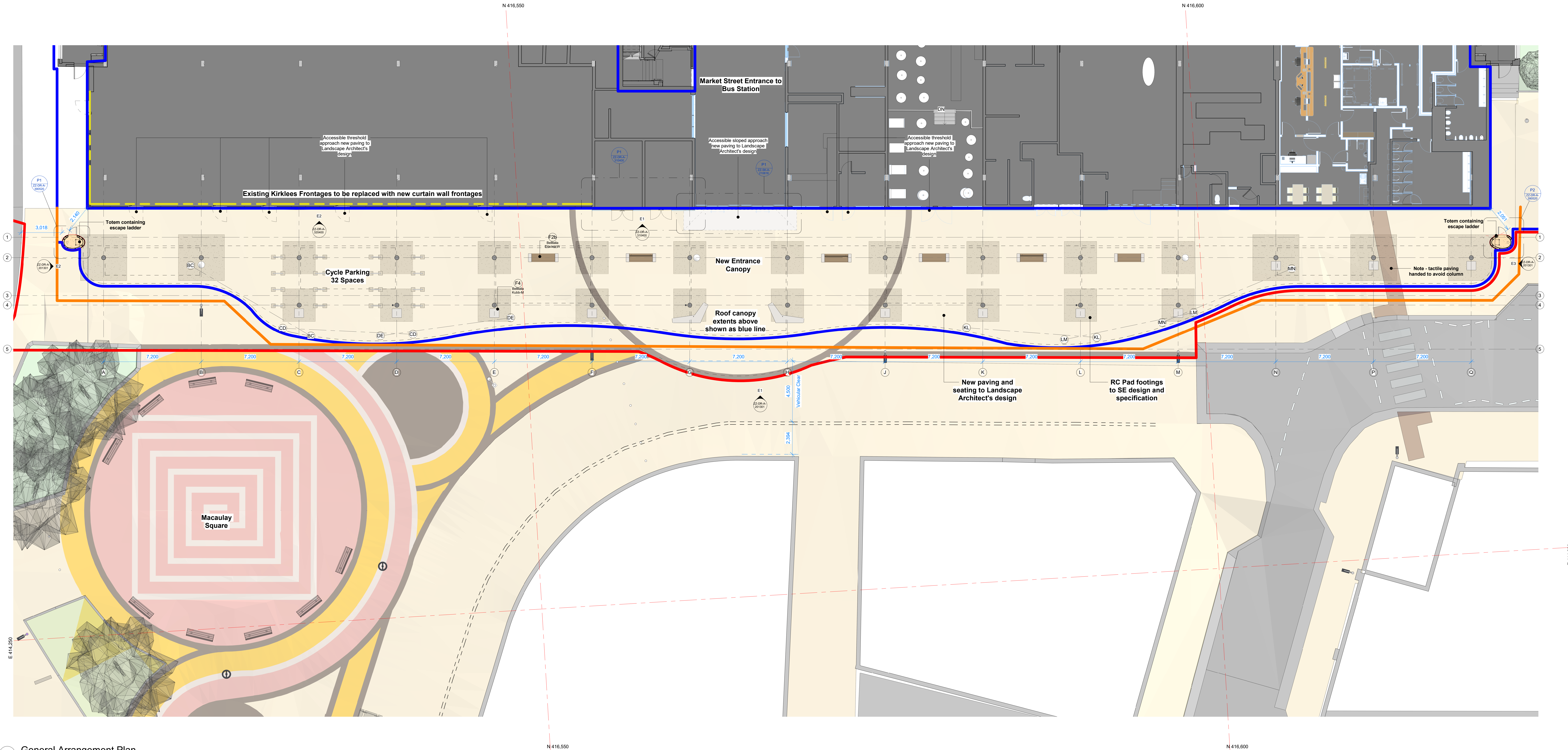
1 General Arrangement Plan Scale: 1 : 100
