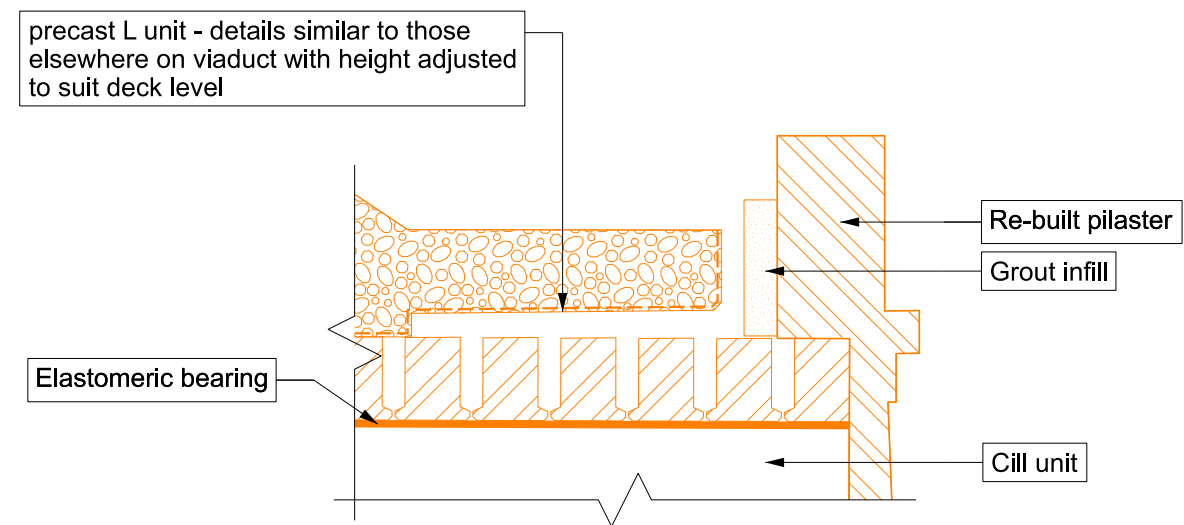
Section M-M Scale 1:50
