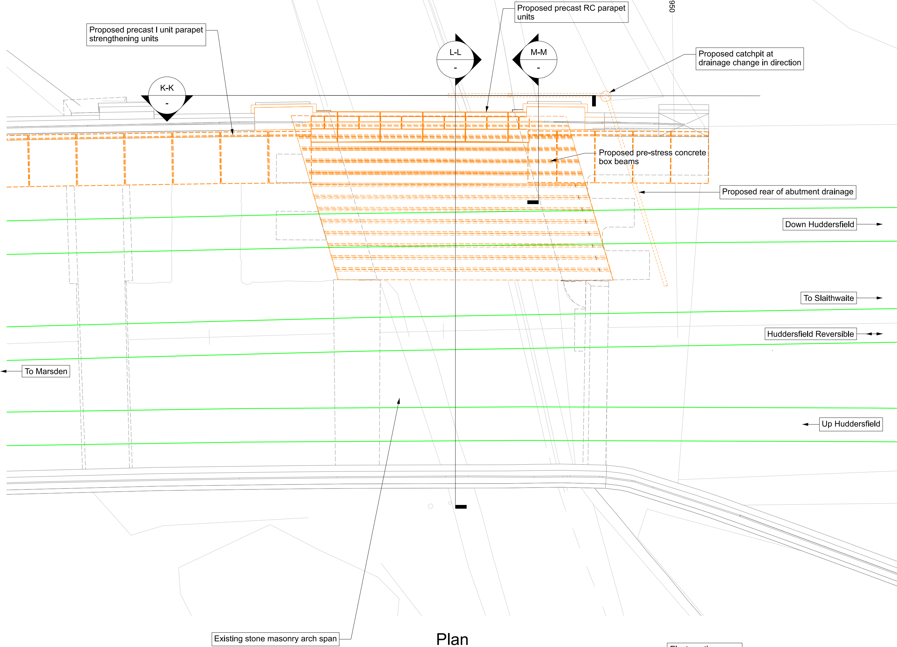
Plan Scale 1:100
