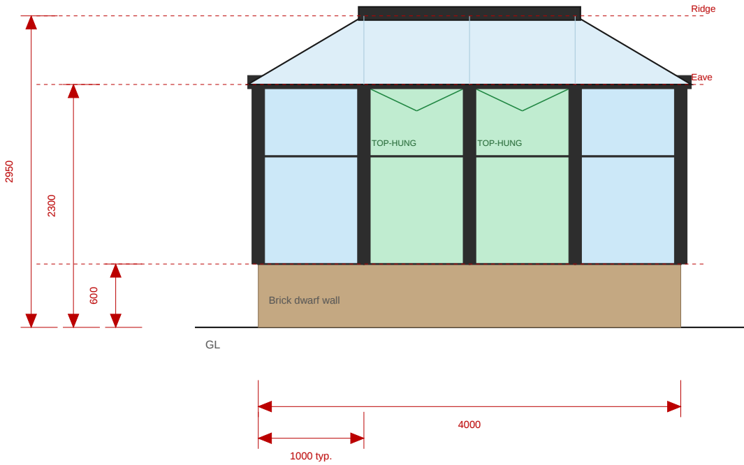
RIGHT SIDE ELEVATION — 1:50
