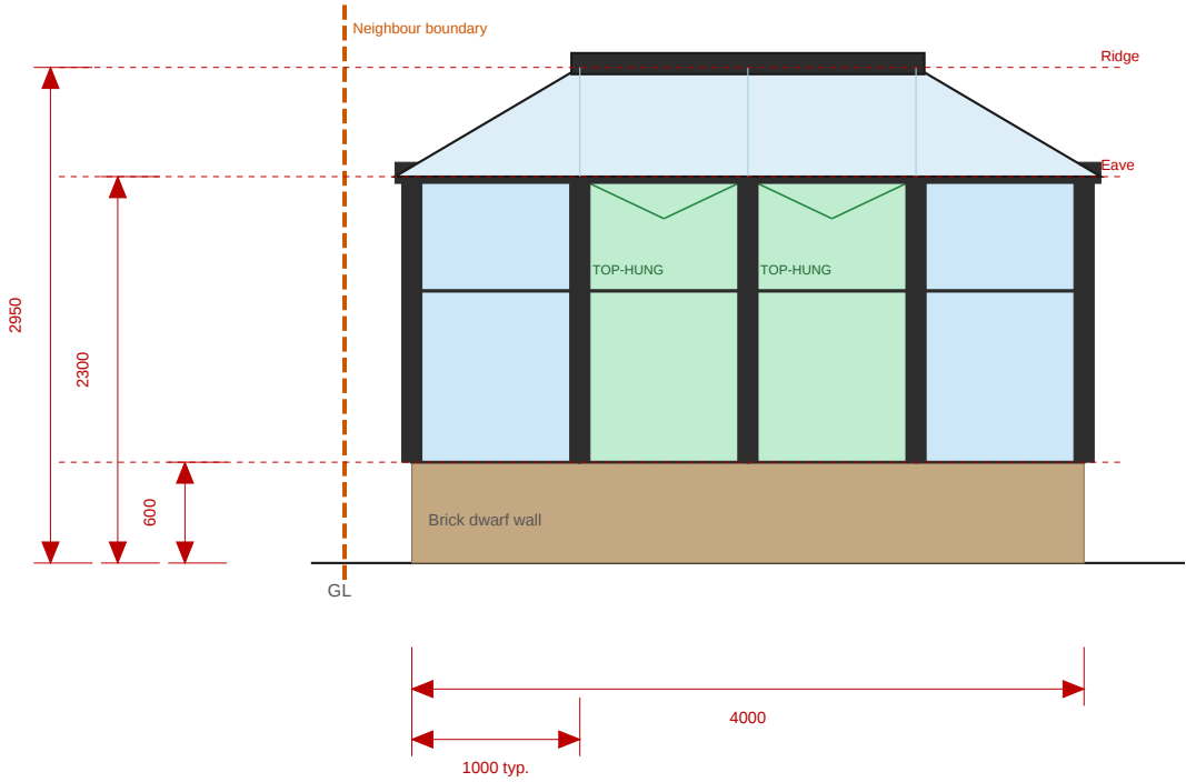
LEFT SIDE ELEVATION (neighbour boundary) — 1:50
