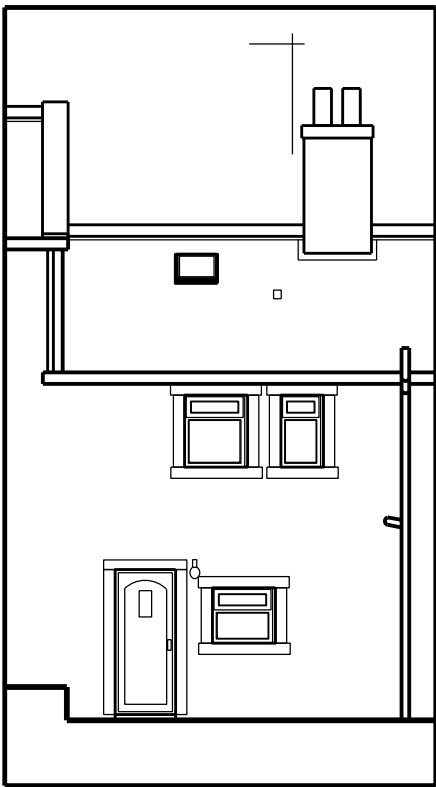
North Elevation
