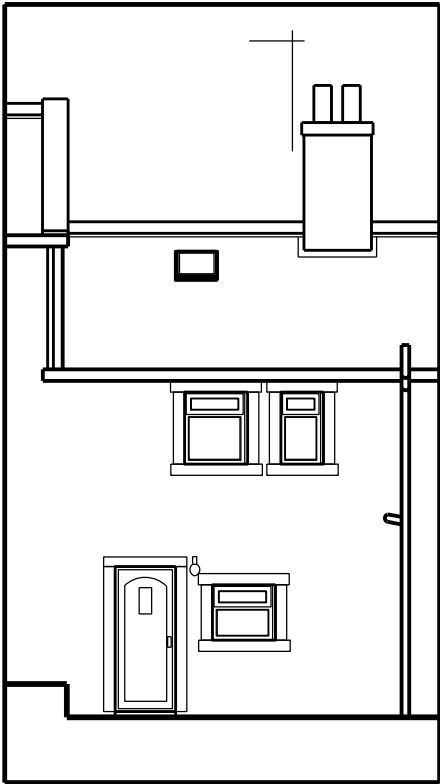
North Elevation
