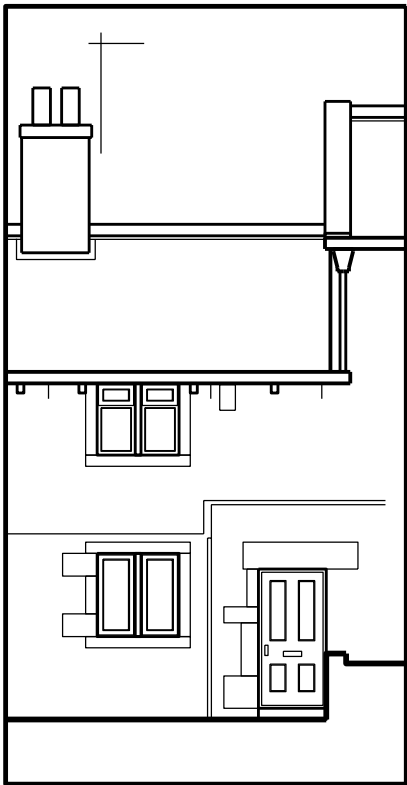
South Elevation
