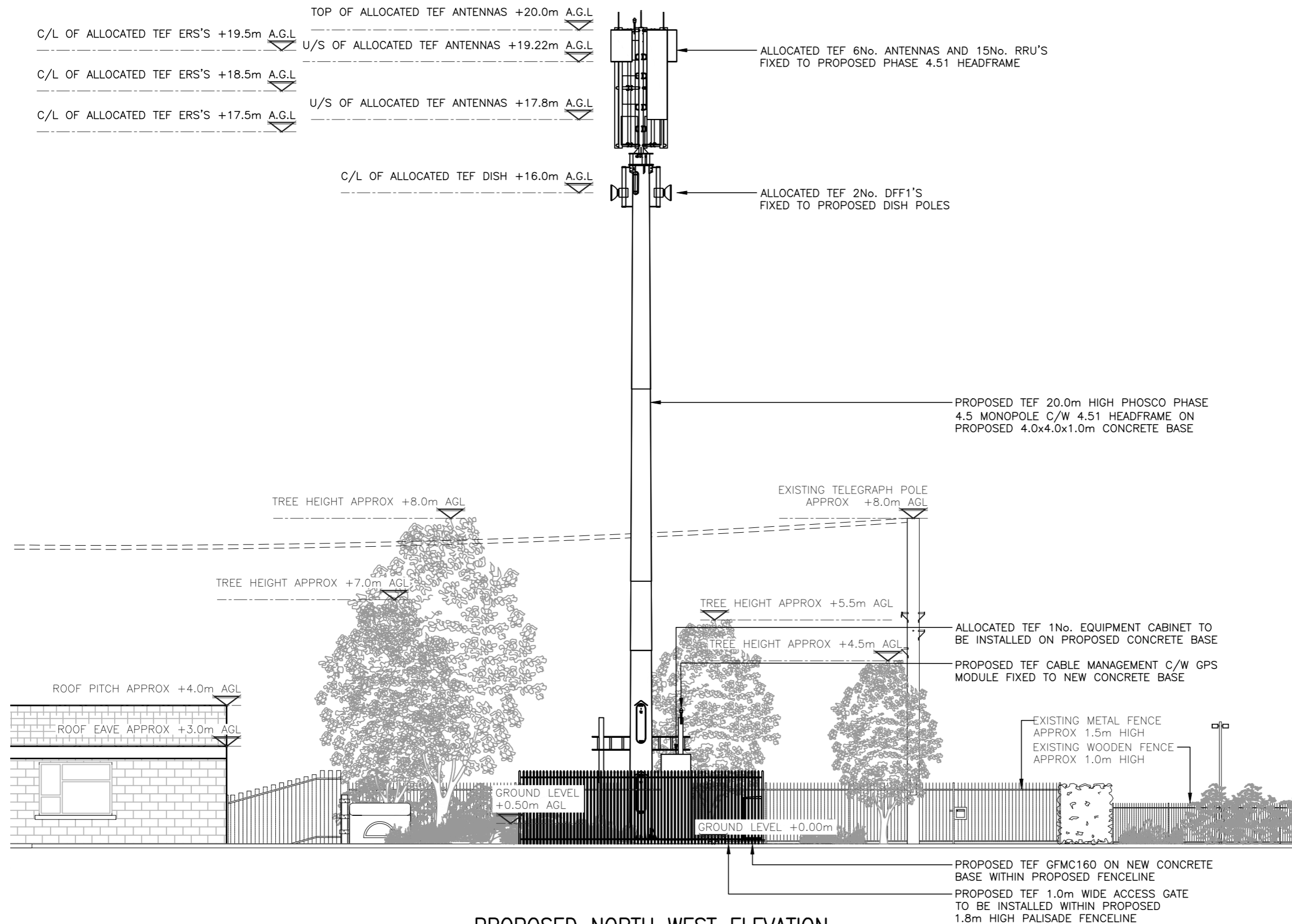
PROPOSED NORTH WEST ELEVATION
