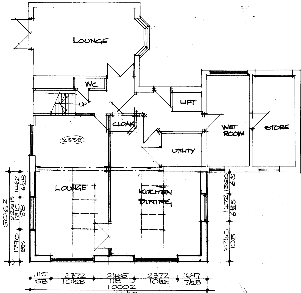
GROUND 1:100
