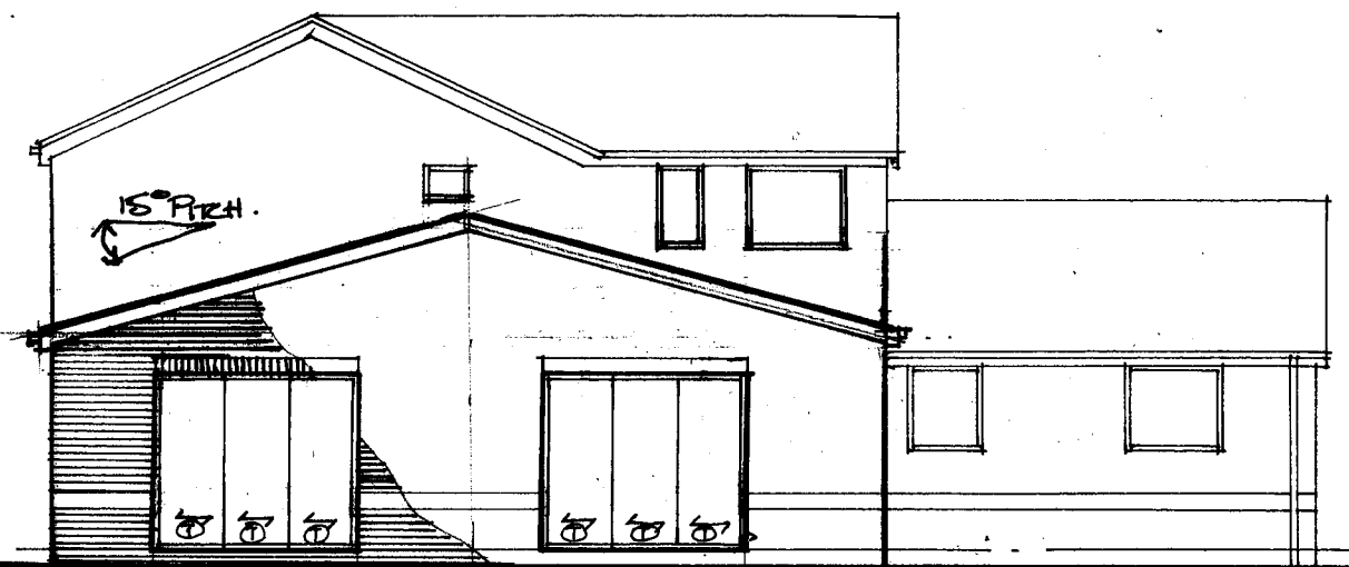
REAR 1:100
