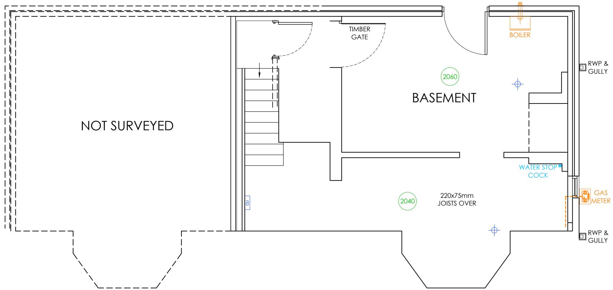
BASEMENT PLAN
