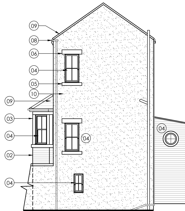
EAST ELEVATION
