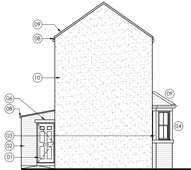
WEST ELEVATION
