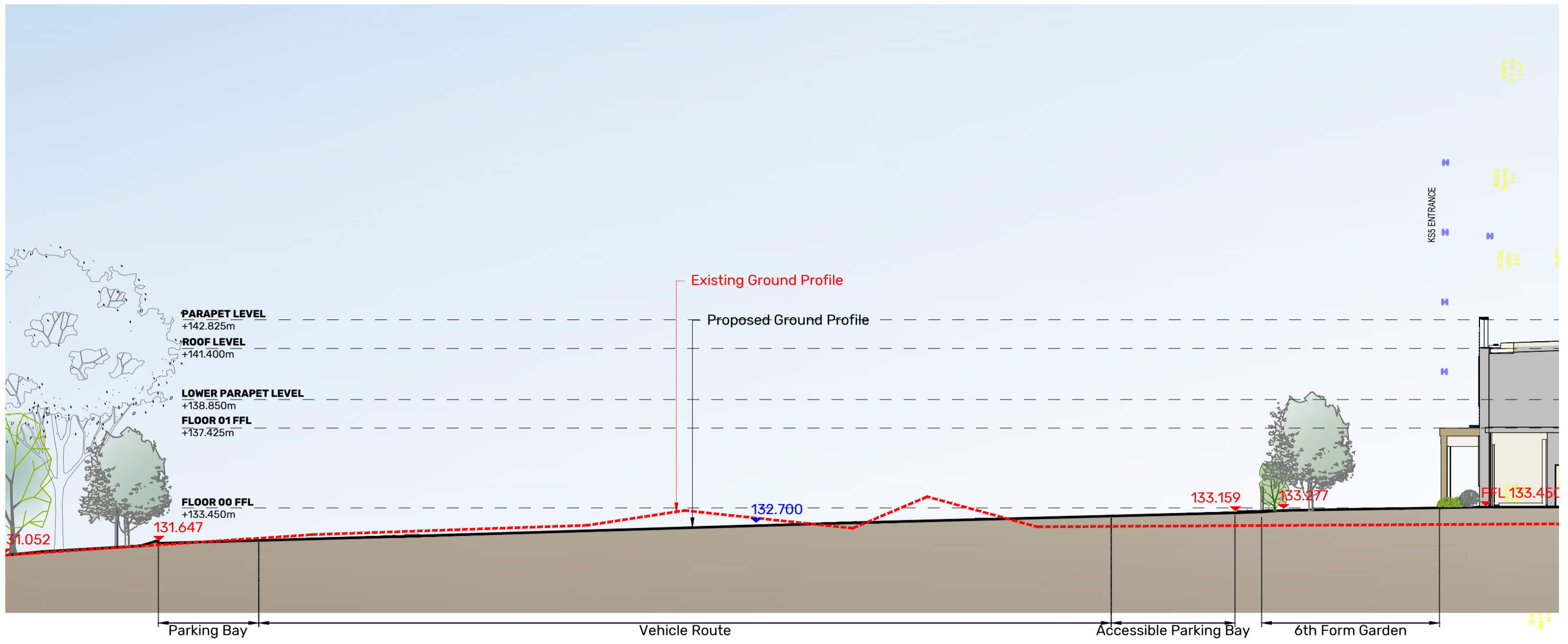
SECTION C-C' Scale 1:200
