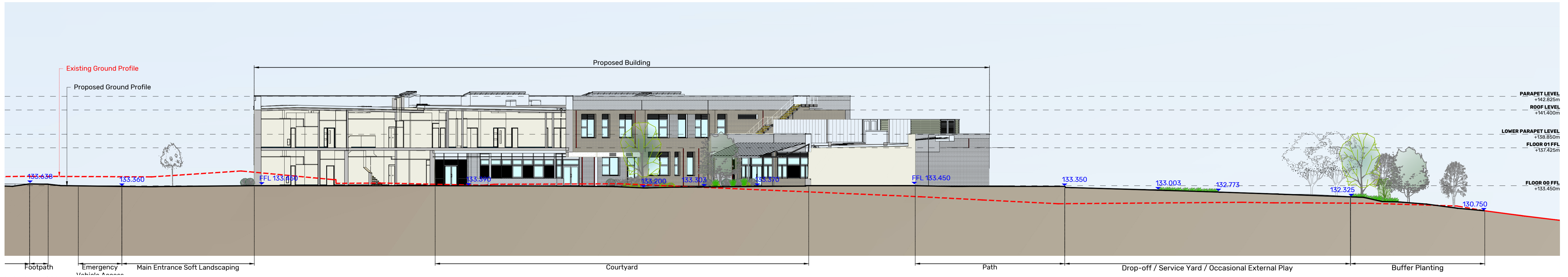
SECTION E-E' 02 Scale 1:200
