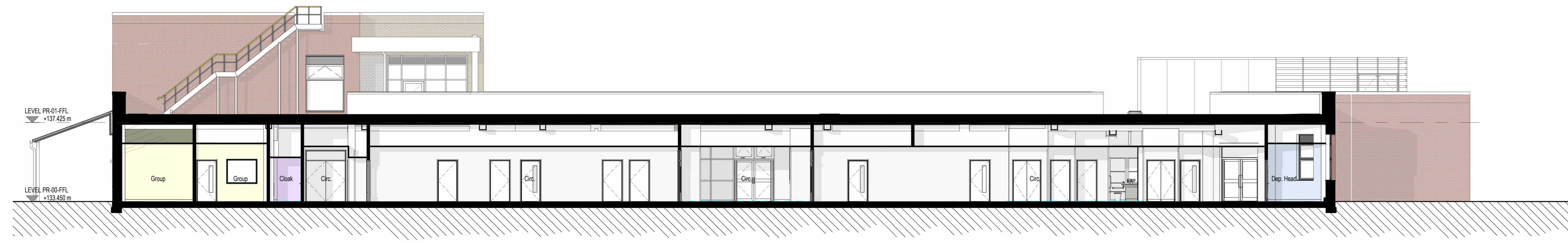
S3 SECTION S3 10120 1 : 100 GA Planning Section - S3
