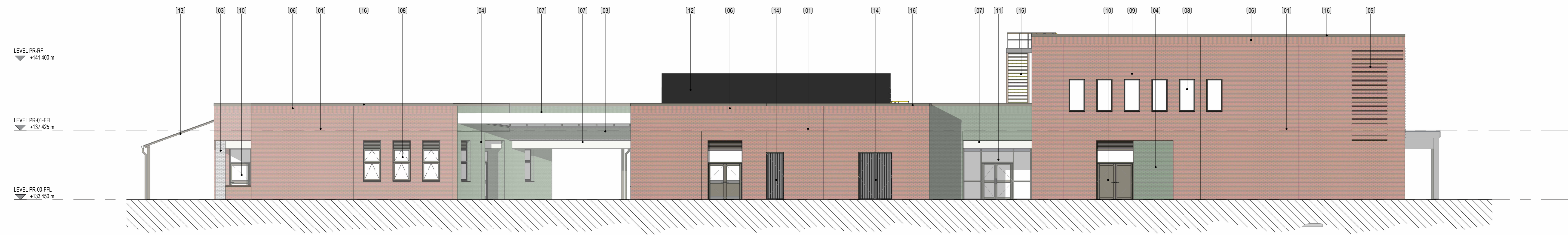
1 ELEVATION 1 10110 1 : 100 GA East Planning Elevation
