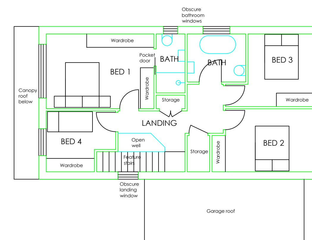
PROPOSED FIRST FLOOR PLAN (new extension)
