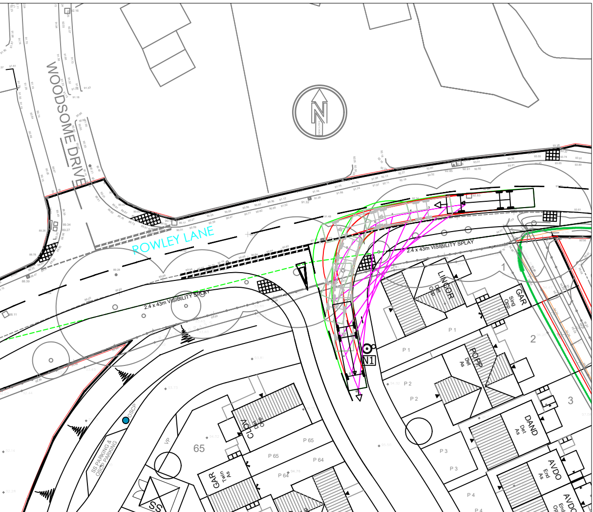
SITE ENTRANCE
