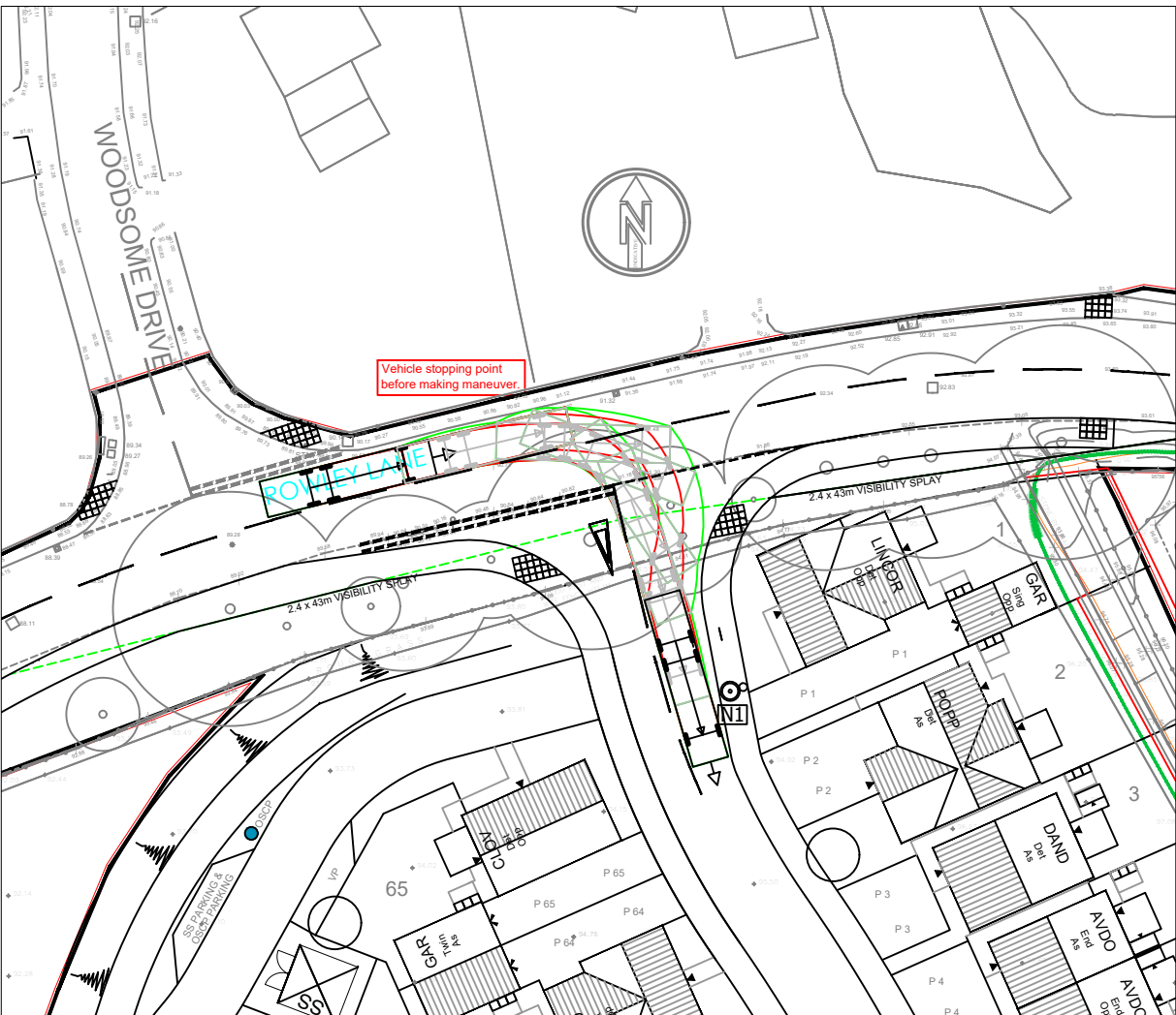
SITE ENTRANCE
