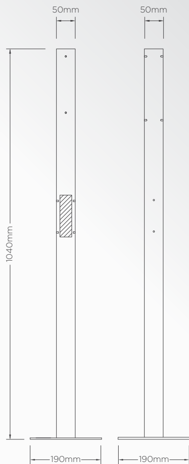
Mounting post:
