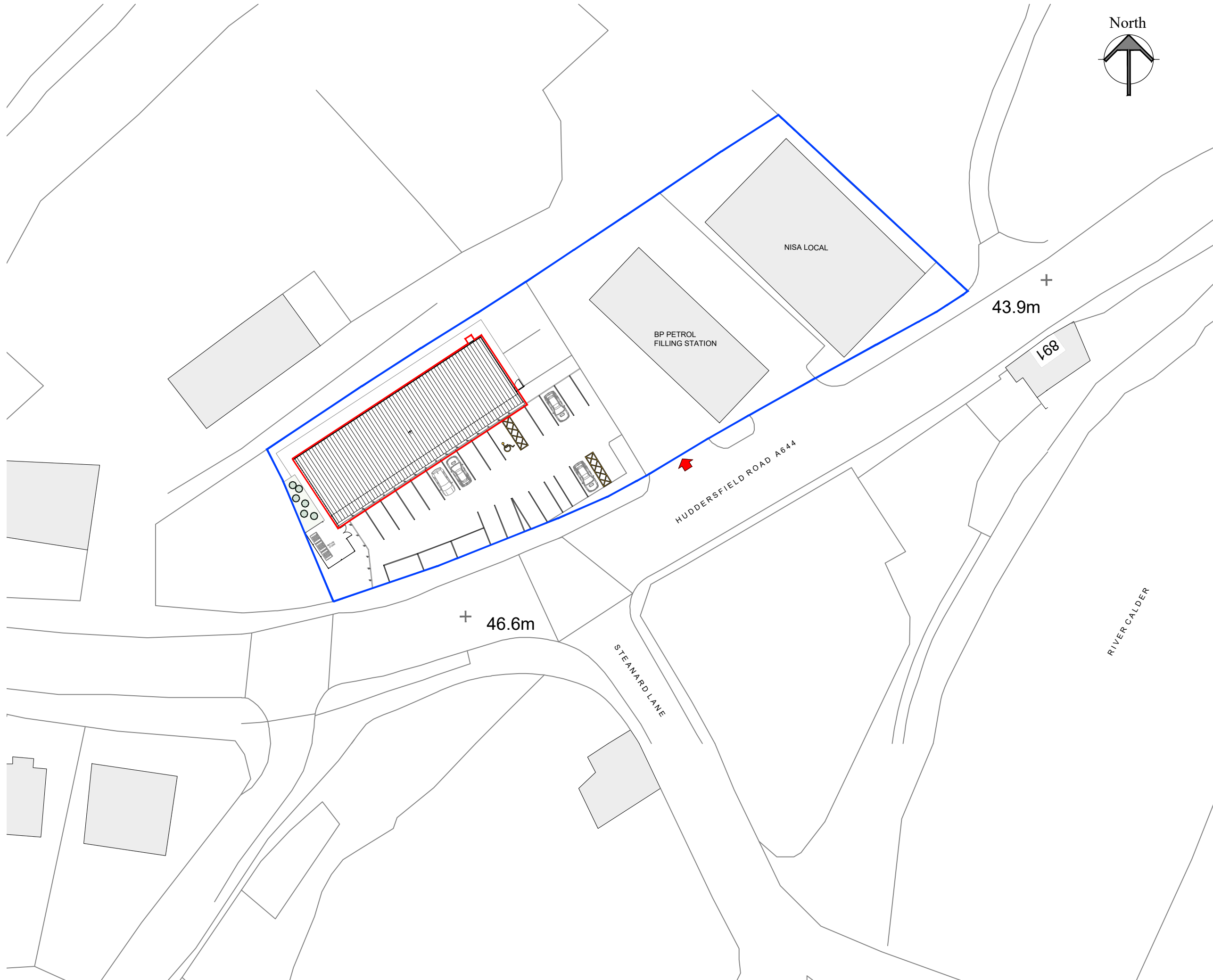
EXISTING BLOCK PLAN | SCALE 1:500
